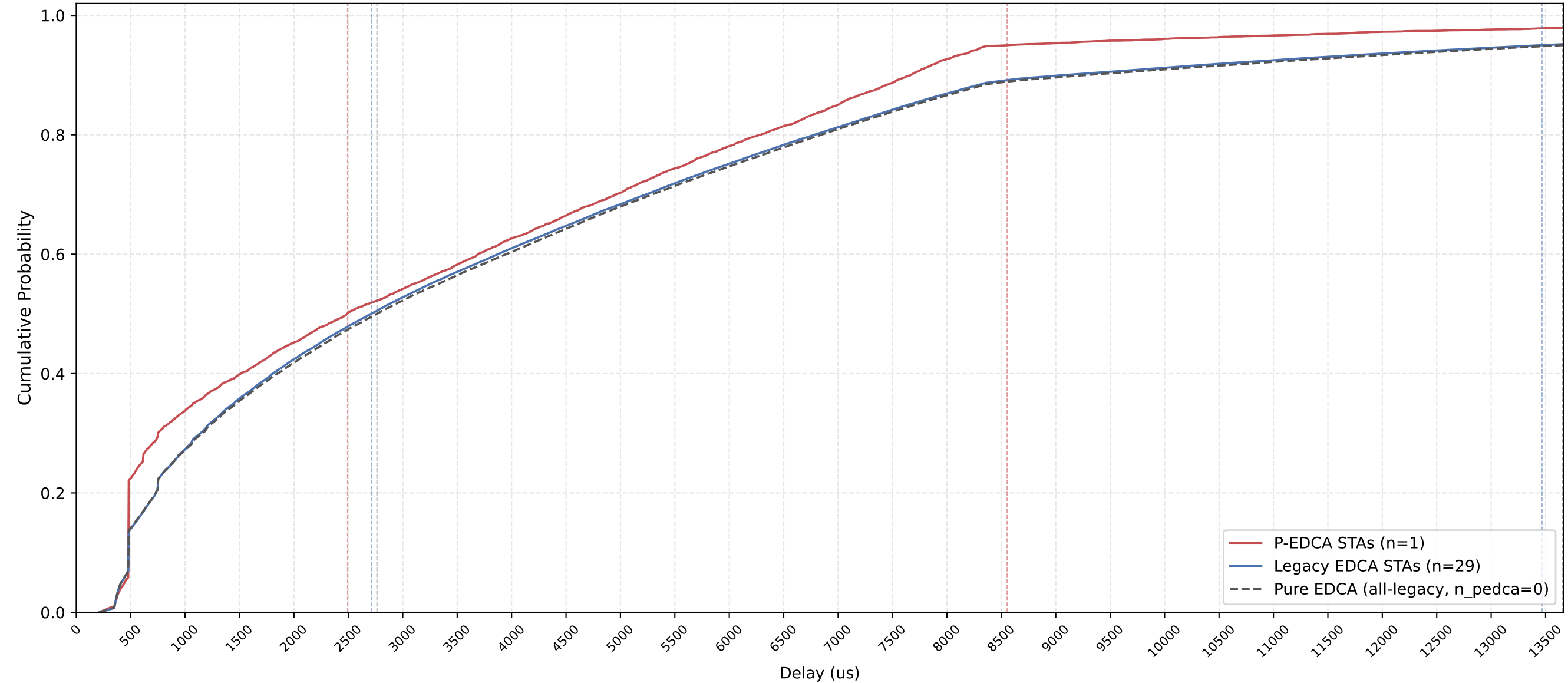
P-EDCA vs Legacy Delay CDF — n_pedca=1, n_legacy=29, nSta=30, 1Mbps, avg of 10 runs
