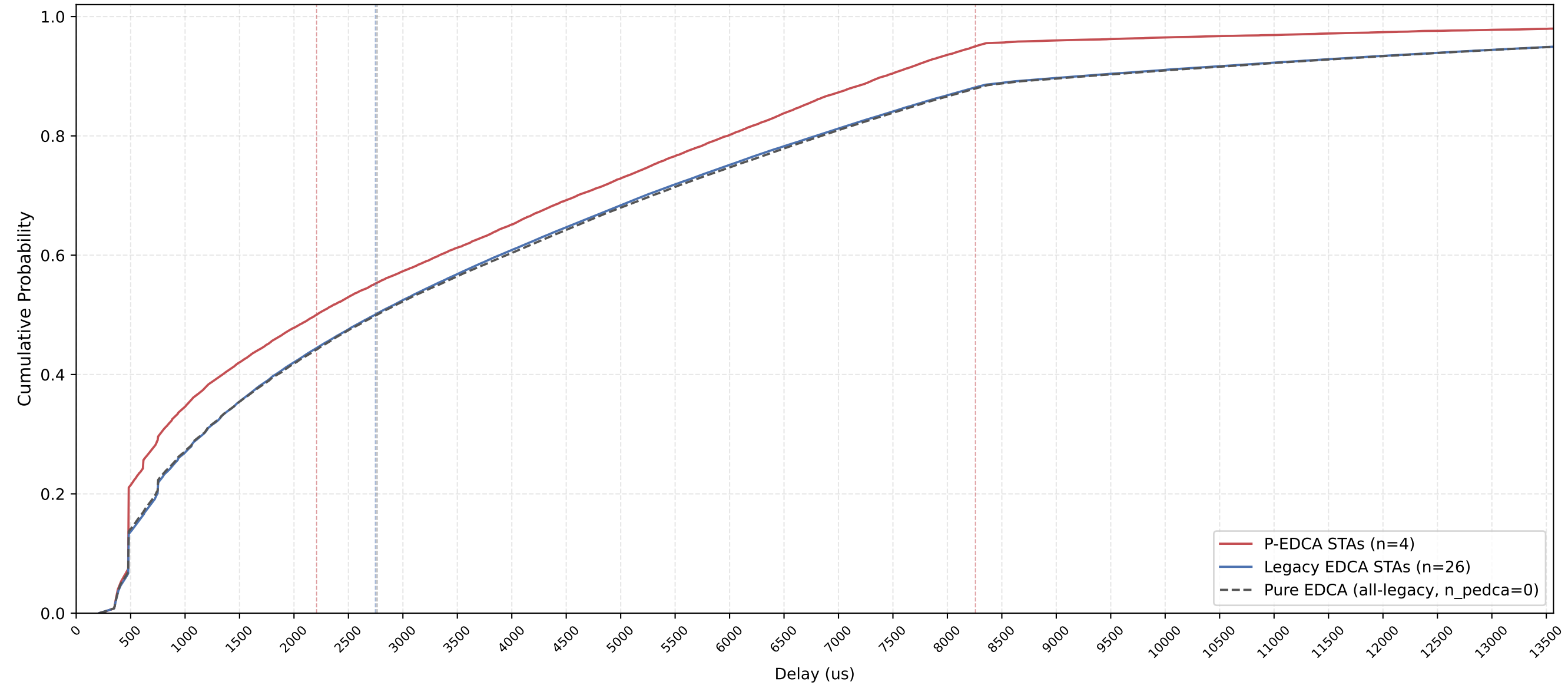
P-EDCA vs Legacy Delay CDF — n_pedca=4, n_legacy=26, nSta=30, 1Mbps, avg of 10 runs
