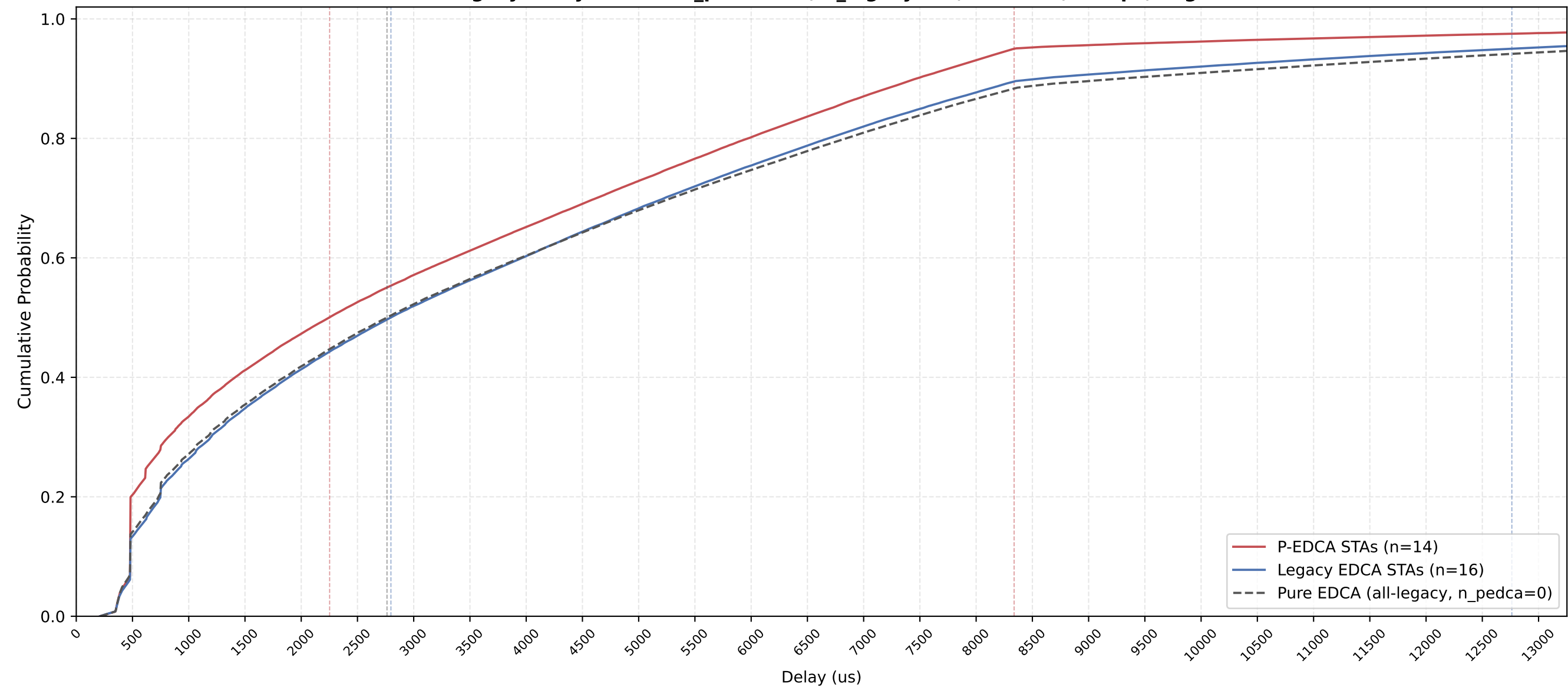
P-EDCA vs Legacy Delay CDF — n_pedca=14, n_legacy=16, nSta=30, 1Mbps, avg of 10 runs
