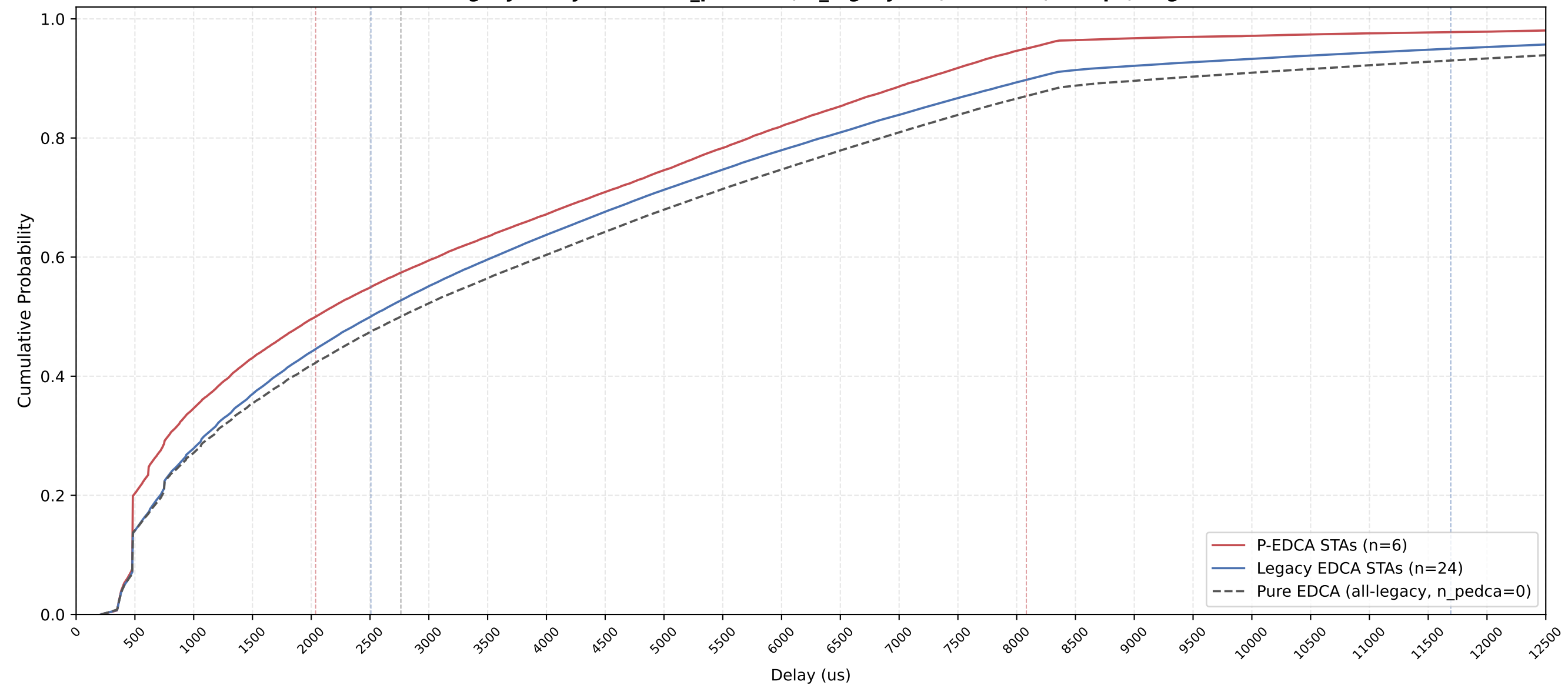
P-EDCA vs Legacy Delay CDF — n_pedca=6, n_legacy=24, nSta=30, 1Mbps, avg of 10 runs
