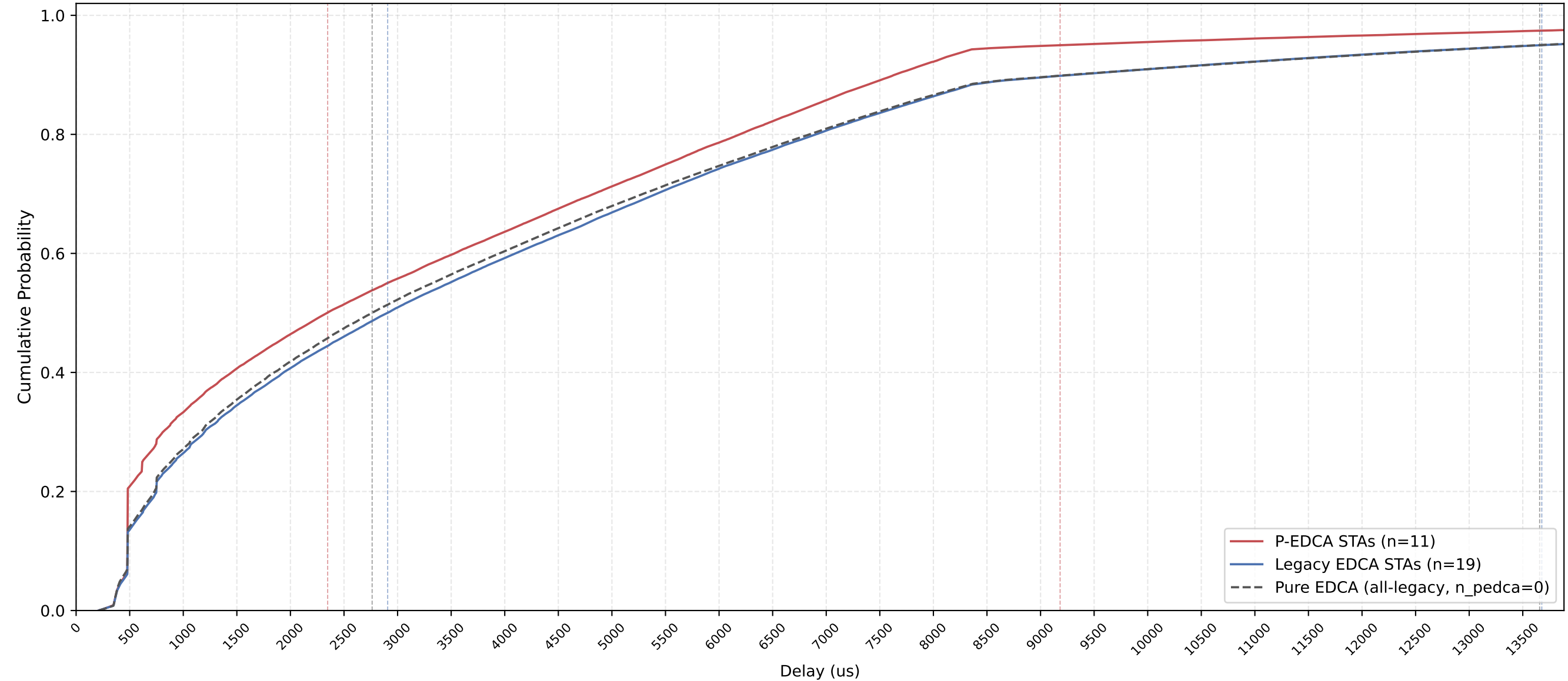
P-EDCA vs Legacy Delay CDF — n_pedca=11, n_legacy=19, nSta=30, 1Mbps, avg of 10 runs
