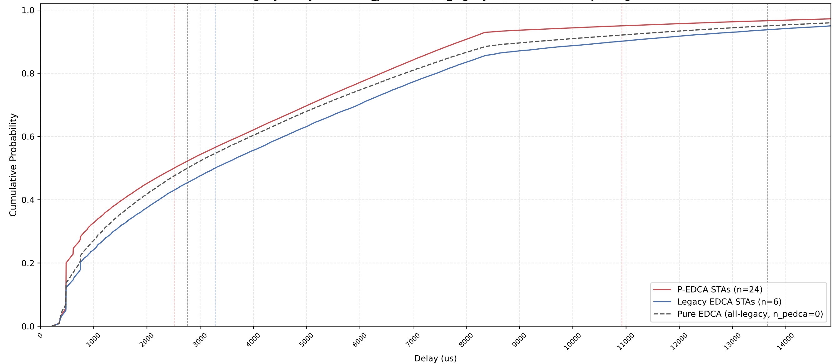
P-EDCA vs Legacy Delay CDF — n_pedca=24, n_legacy=6, nSta=30, 1Mbps, avg of 10 runs
