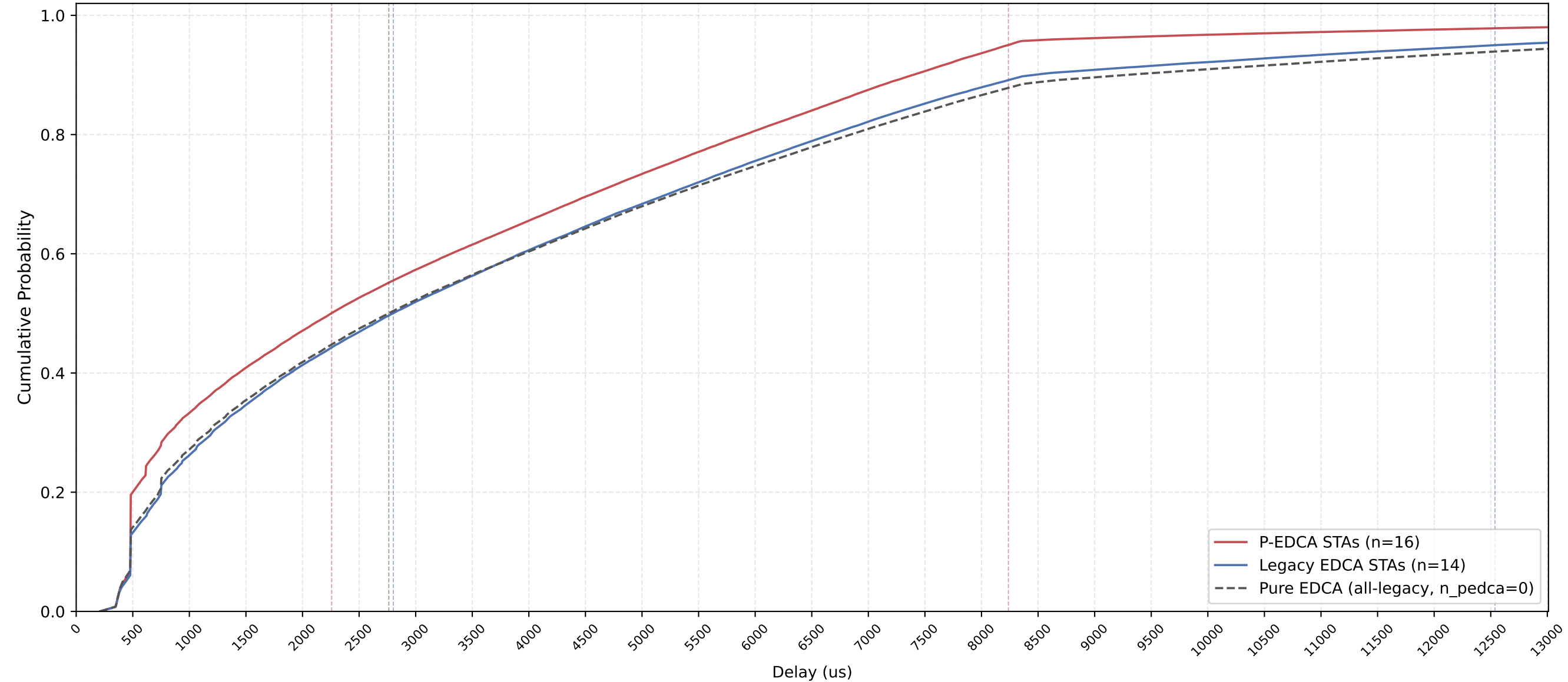
P-EDCA vs Legacy Delay CDF — n_pedca=16, n_legacy=14, nSta=30, 1Mbps, avg of 10 runs
