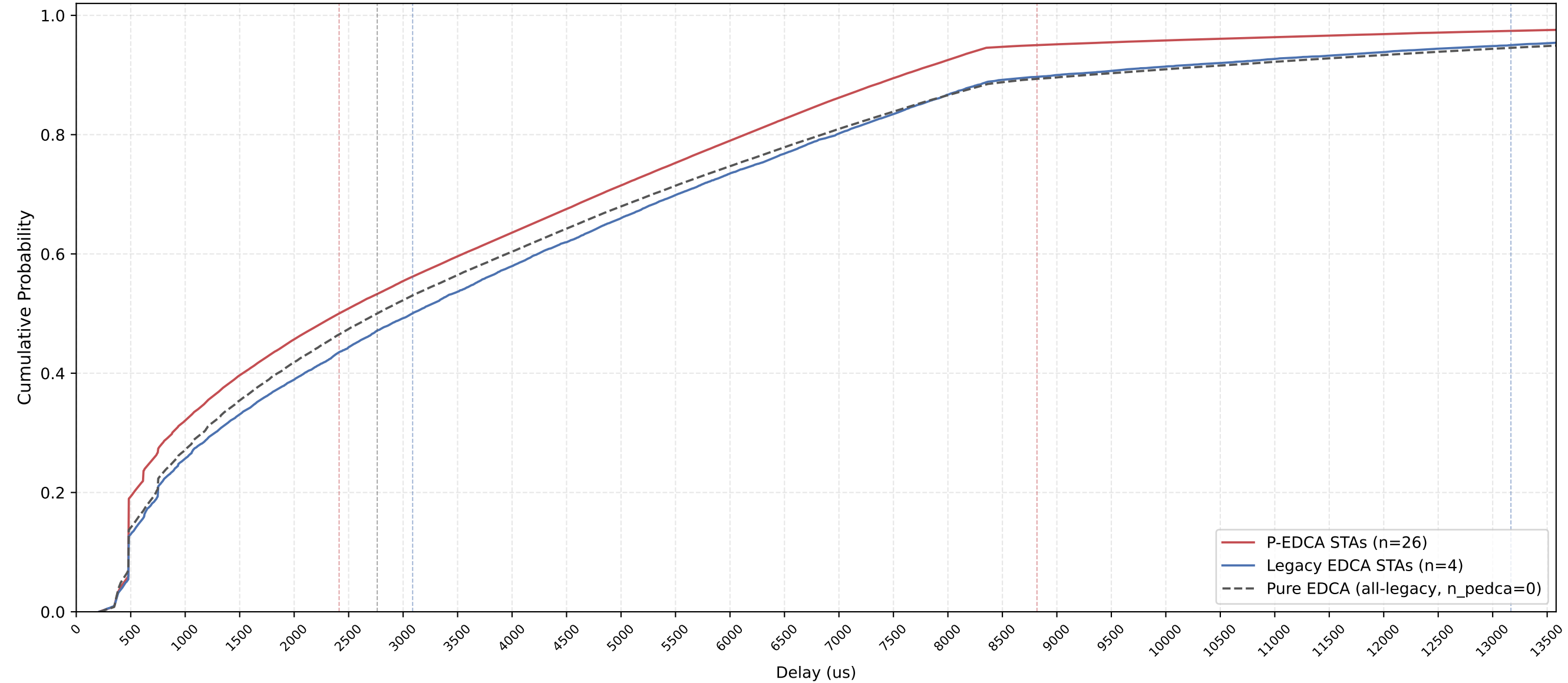
P-EDCA vs Legacy Delay CDF — n_pedca=26, n_legacy=4, nSta=30, 1Mbps, avg of 10 runs
