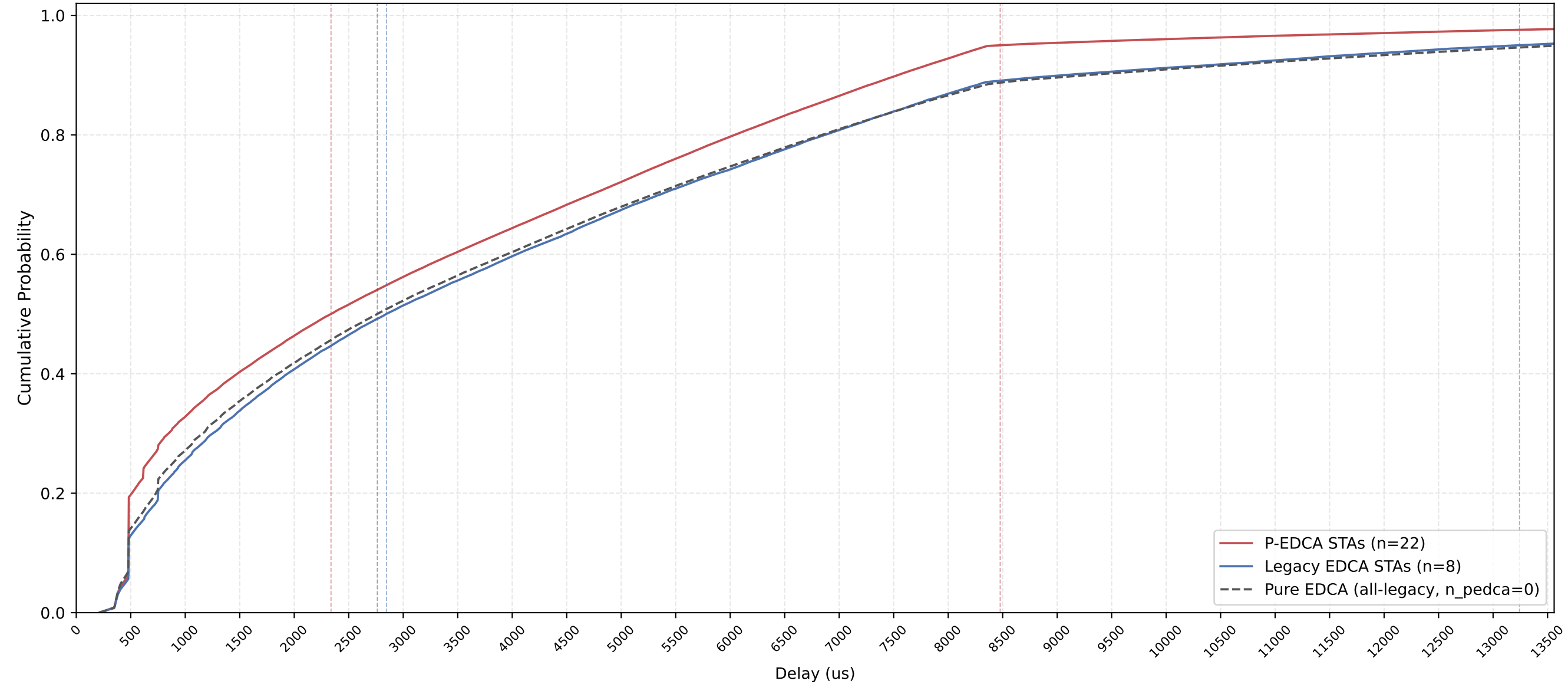
P-EDCA vs Legacy Delay CDF — n_pedca=22, n_legacy=8, nSta=30, 1Mbps, avg of 10 runs
