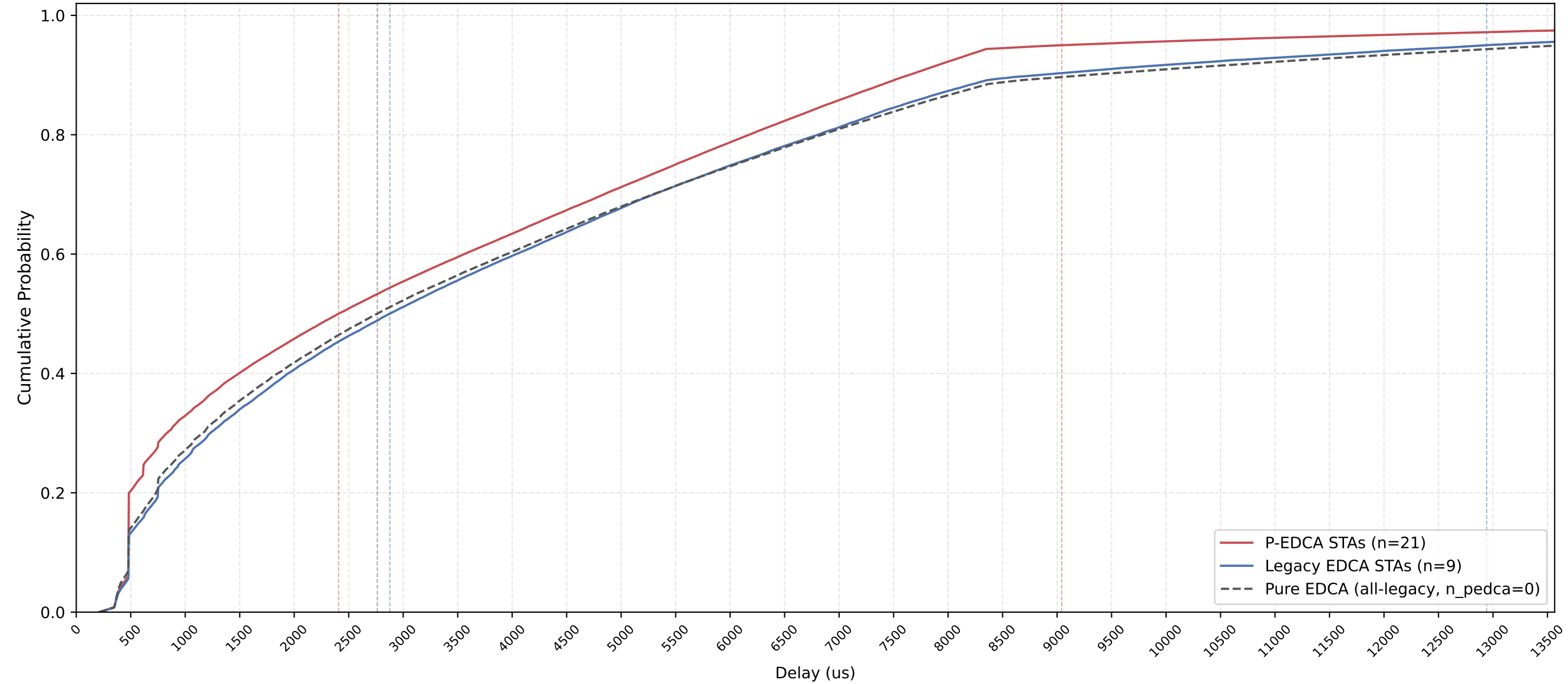
P-EDCA vs Legacy Delay CDF — n_pedca=21, n_legacy=9, nSta=30, 1Mbps, avg of 10 runs
