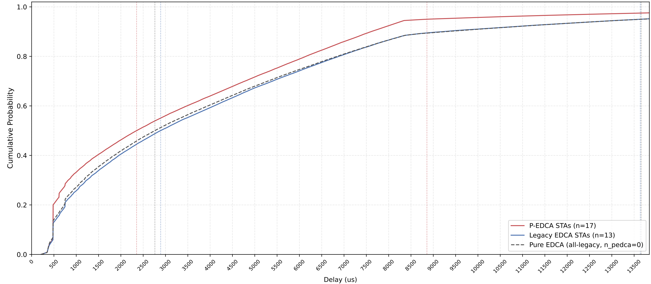
P-EDCA vs Legacy Delay CDF — n_pedca=17, n_legacy=13, nSta=30, 1Mbps, avg of 10 runs
