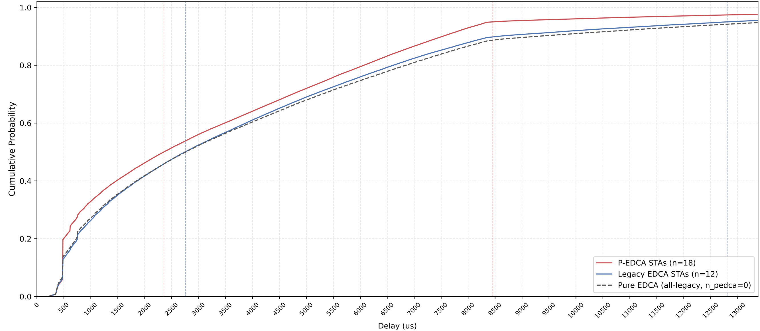
P-EDCA vs Legacy Delay CDF — n_pedca=18, n_legacy=12, nSta=30, 1Mbps, avg of 10 runs
