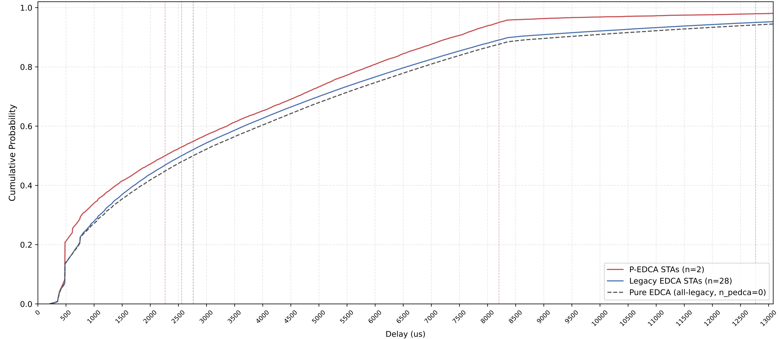
P-EDCA vs Legacy Delay CDF — n_pedca=2, n_legacy=28, nSta=30, 1Mbps, avg of 10 runs
