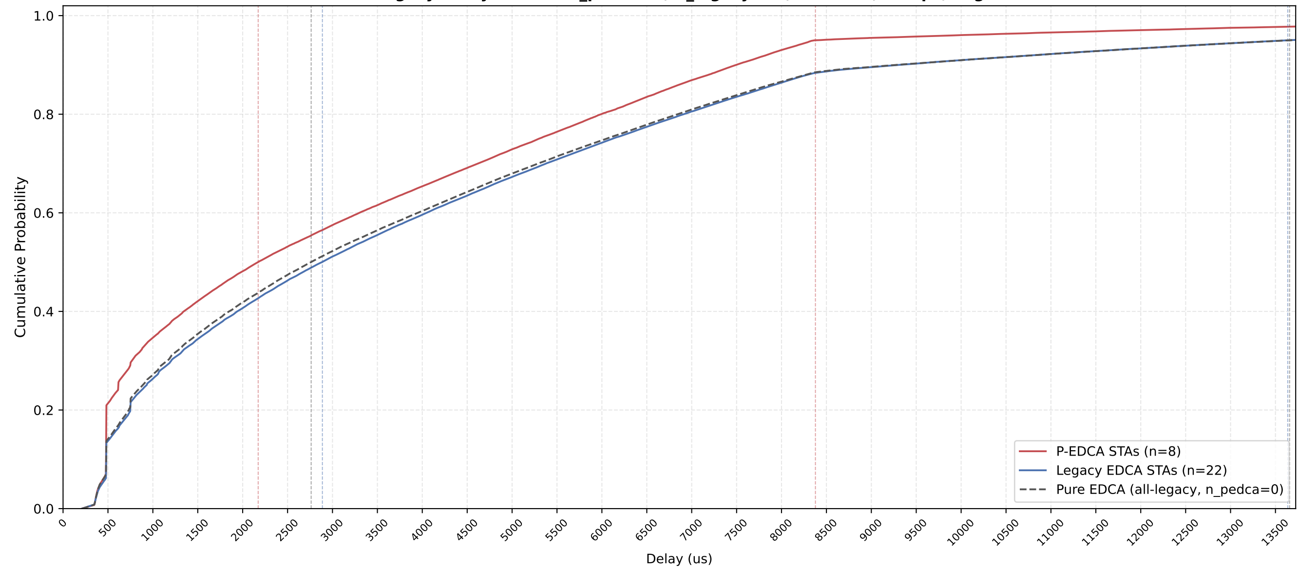
P-EDCA vs Legacy Delay CDF — n_pedca=8, n_legacy=22, nSta=30, 1Mbps, avg of 10 runs
