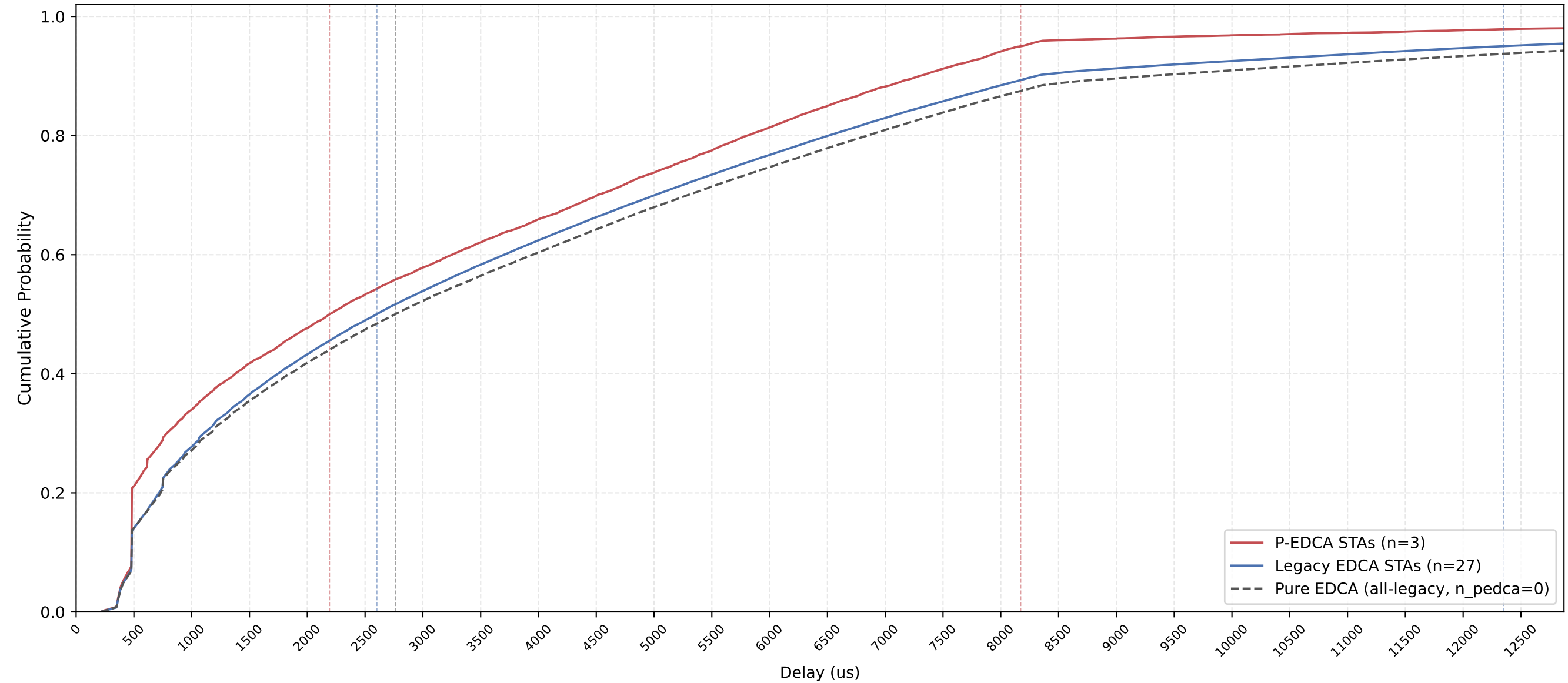
P-EDCA vs Legacy Delay CDF — n_pedca=3, n_legacy=27, nSta=30, 1Mbps, avg of 10 runs
