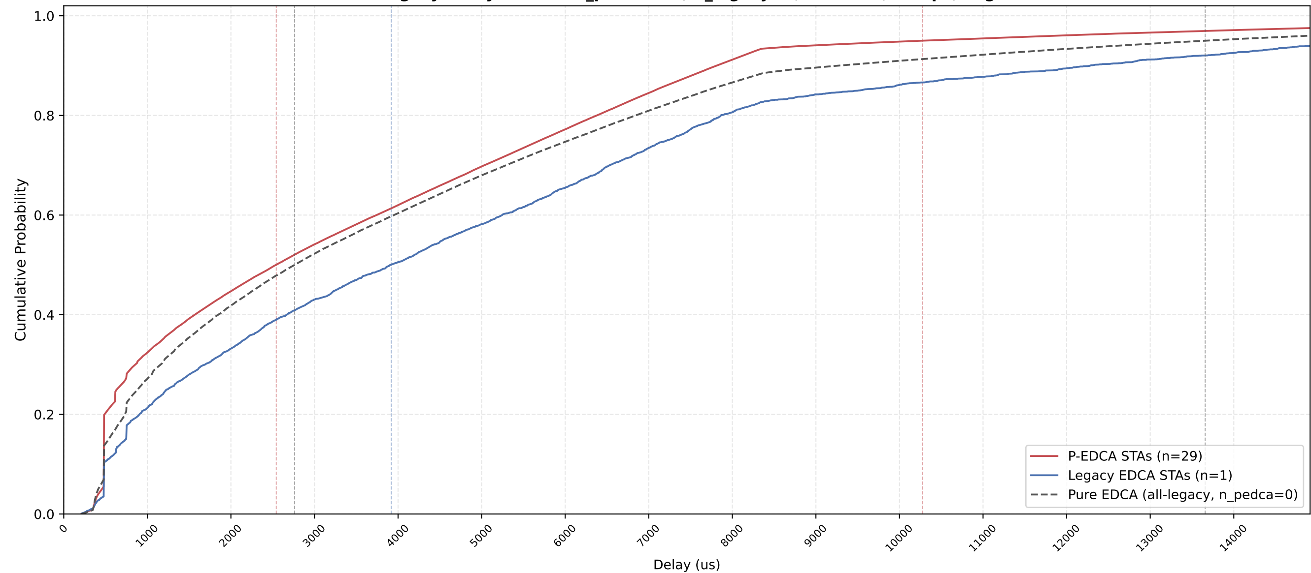
P-EDCA vs Legacy Delay CDF — n_pedca=29, n_legacy=1, nSta=30, 1Mbps, avg of 10 runs
