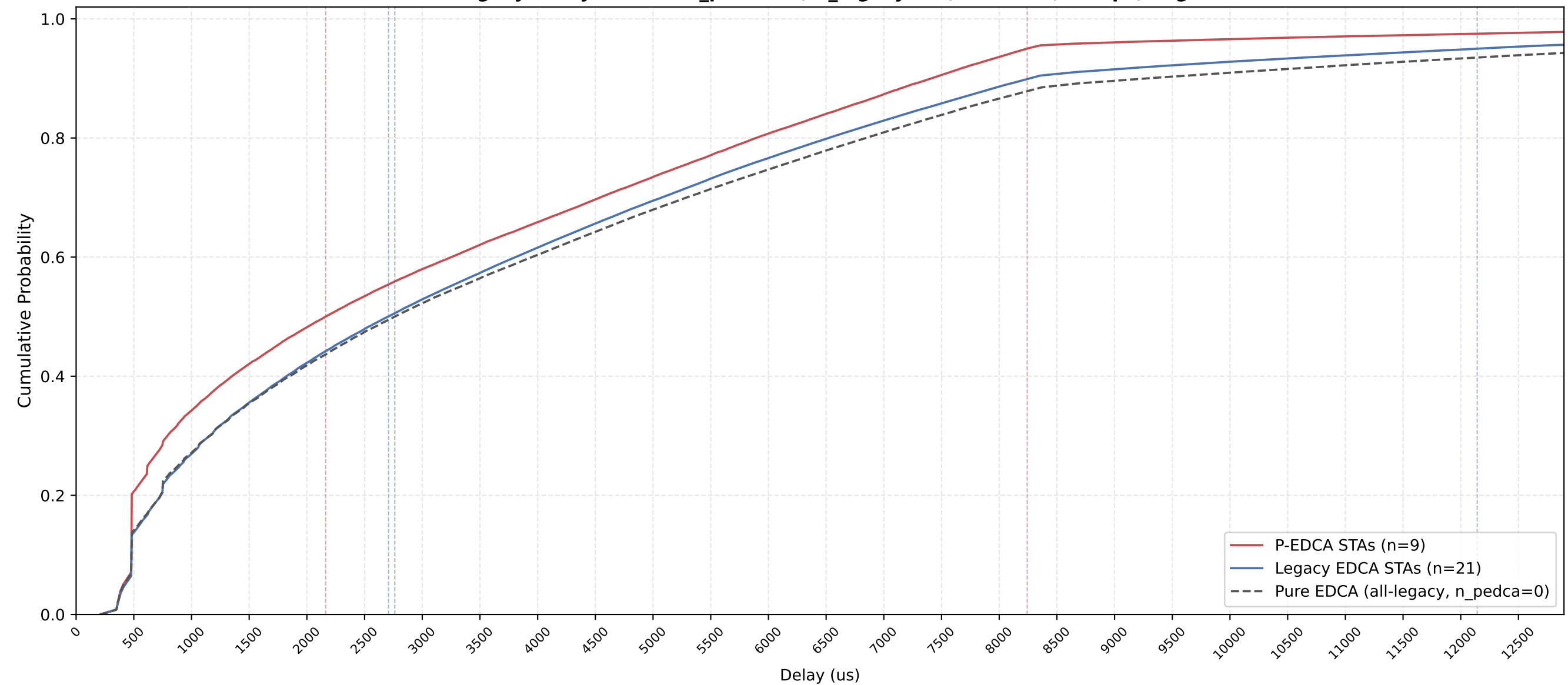
P-EDCA vs Legacy Delay CDF — n_pedca=9, n_legacy=21, nSta=30, 1Mbps, avg of 10 runs
