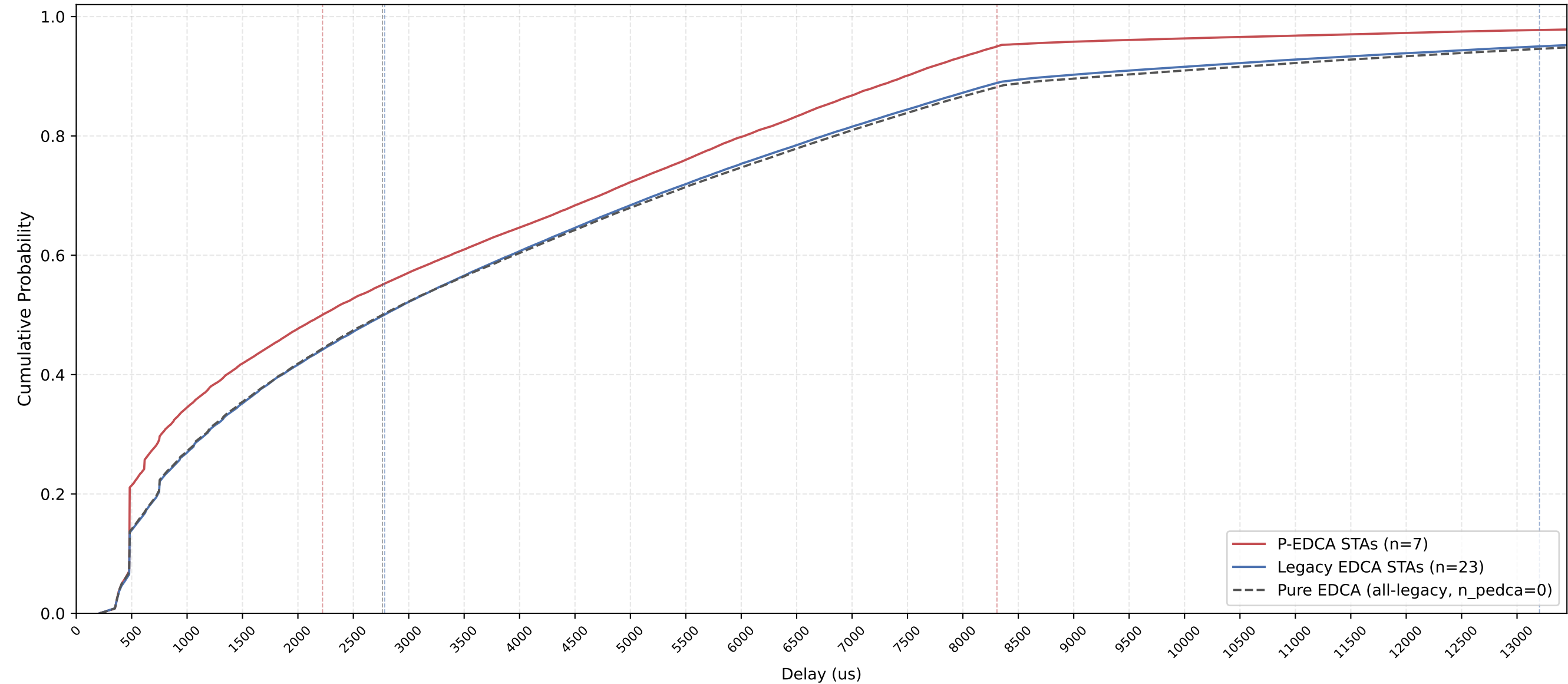
P-EDCA vs Legacy Delay CDF — n_pedca=7, n_legacy=23, nSta=30, 1Mbps, avg of 10 runs
