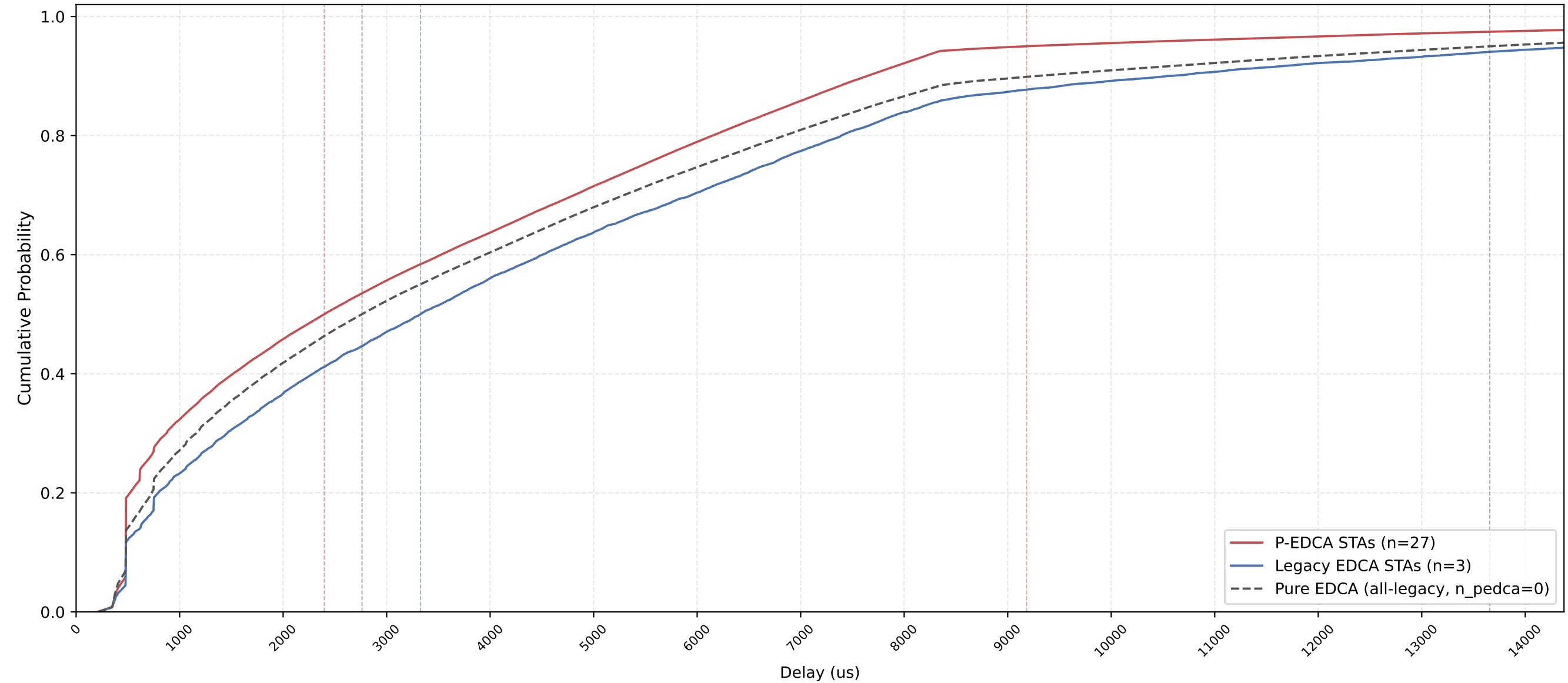
P-EDCA vs Legacy Delay CDF — n_pedca=27, n_legacy=3, nSta=30, 1Mbps, avg of 10 runs
