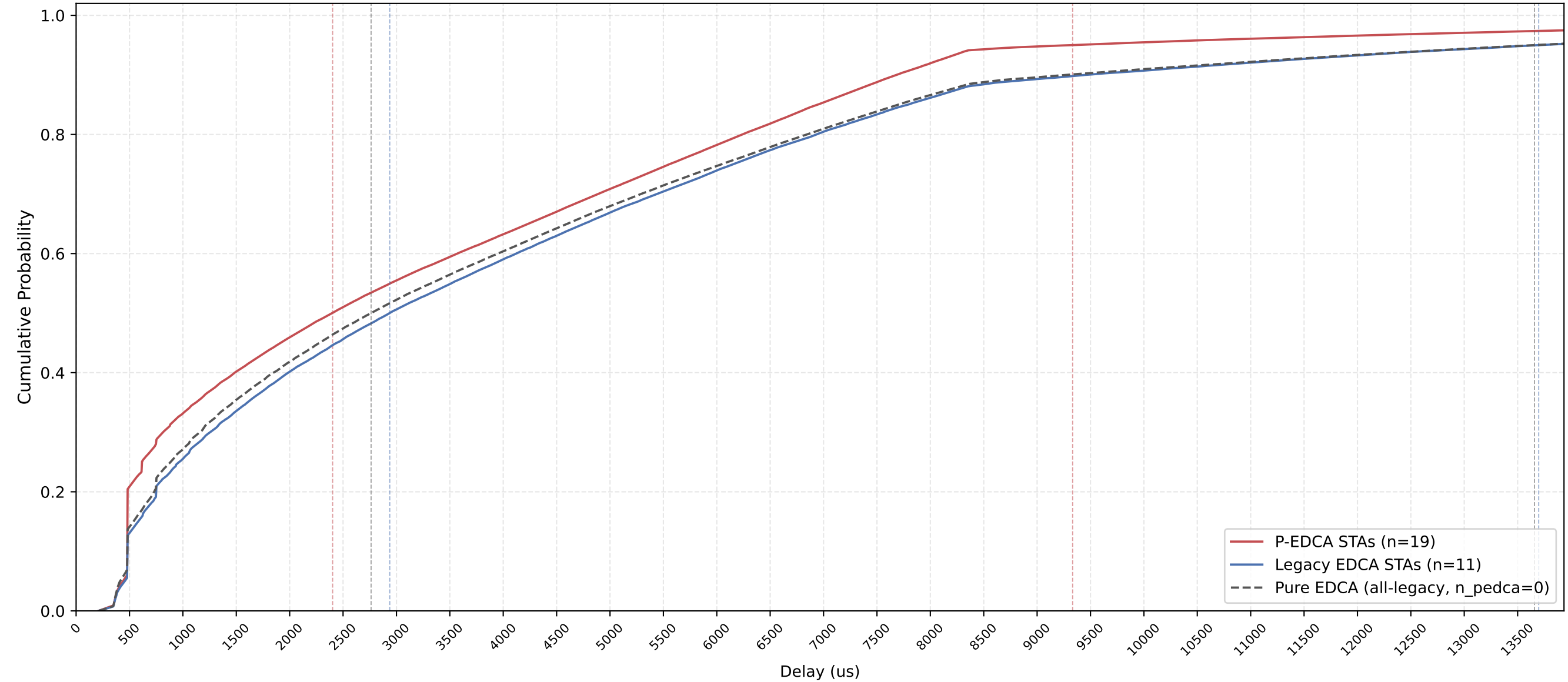
P-EDCA vs Legacy Delay CDF — n_pedca=19, n_legacy=11, nSta=30, 1Mbps, avg of 10 runs
