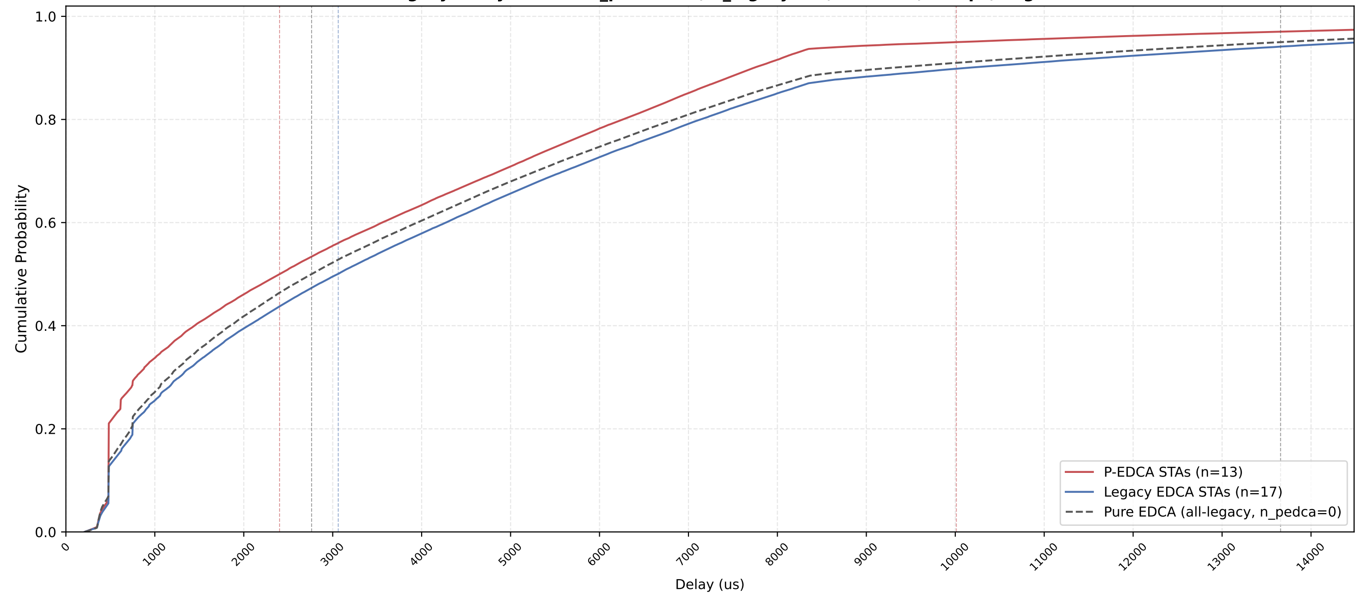
P-EDCA vs Legacy Delay CDF — n_pedca=13, n_legacy=17, nSta=30, 1Mbps, avg of 10 runs
