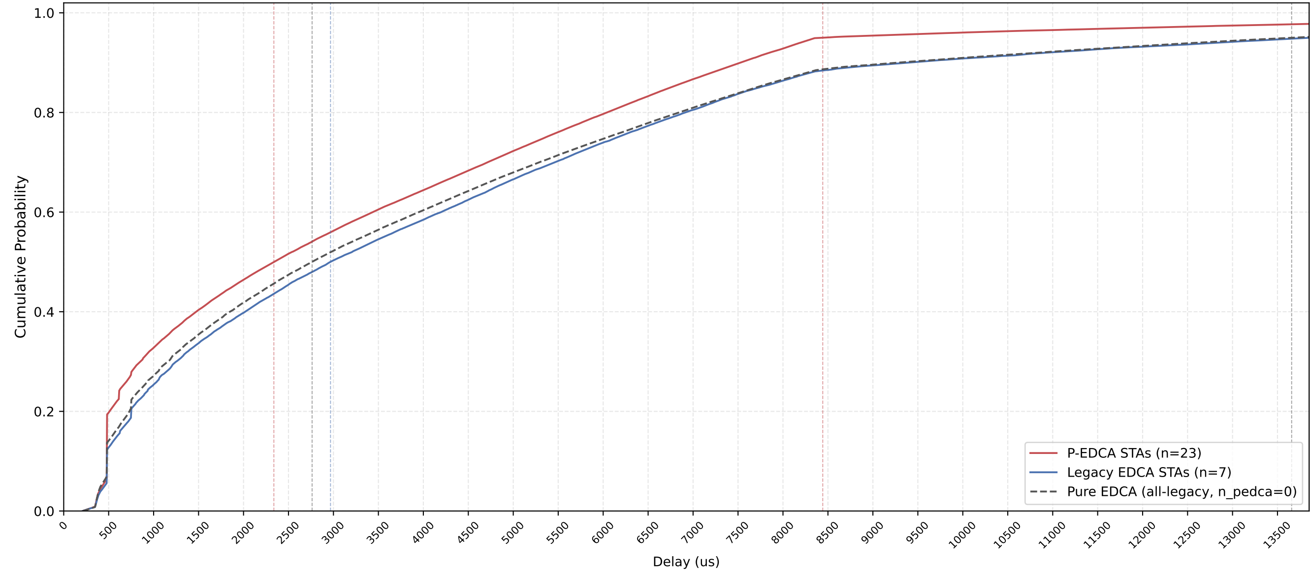
P-EDCA vs Legacy Delay CDF — n_pedca=23, n_legacy=7, nSta=30, 1Mbps, avg of 10 runs
