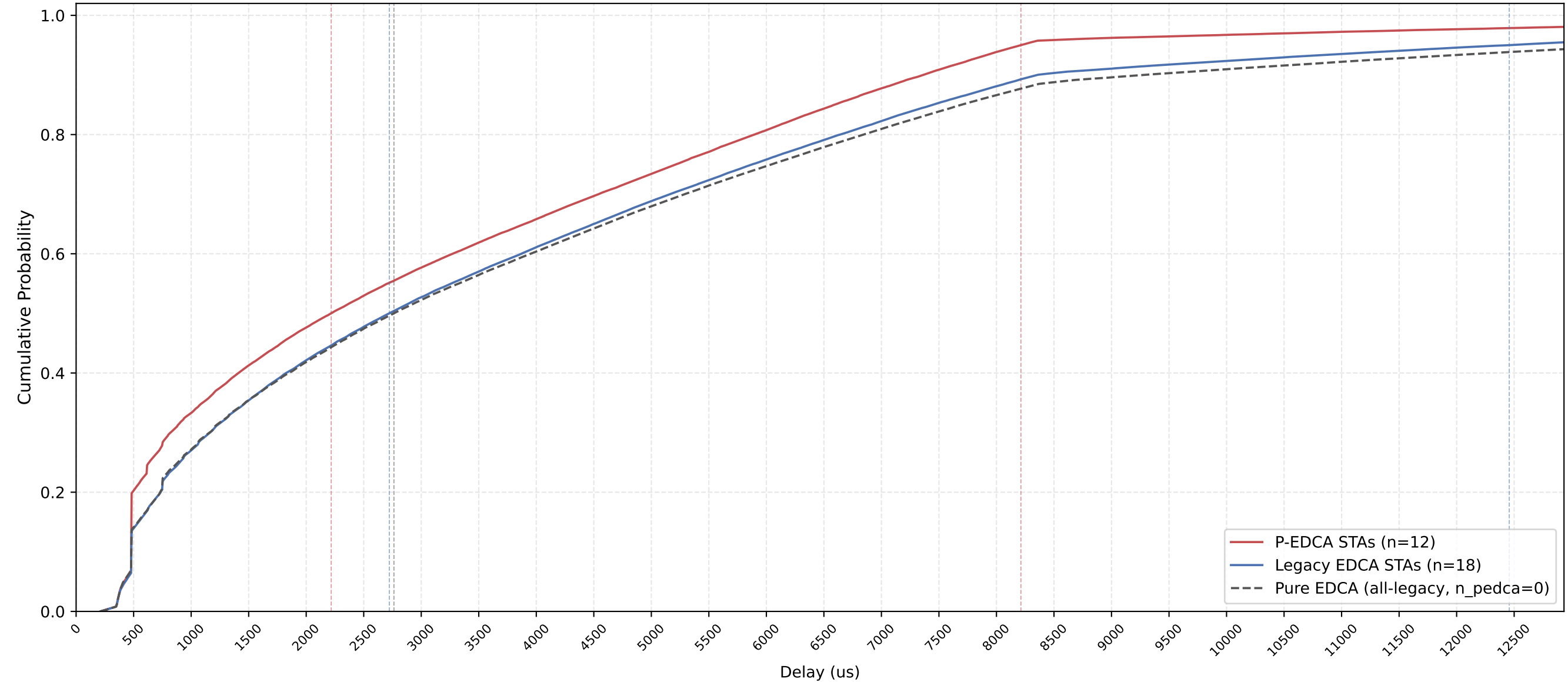
P-EDCA vs Legacy Delay CDF — n_pedca=12, n_legacy=18, nSta=30, 1Mbps, avg of 10 runs
