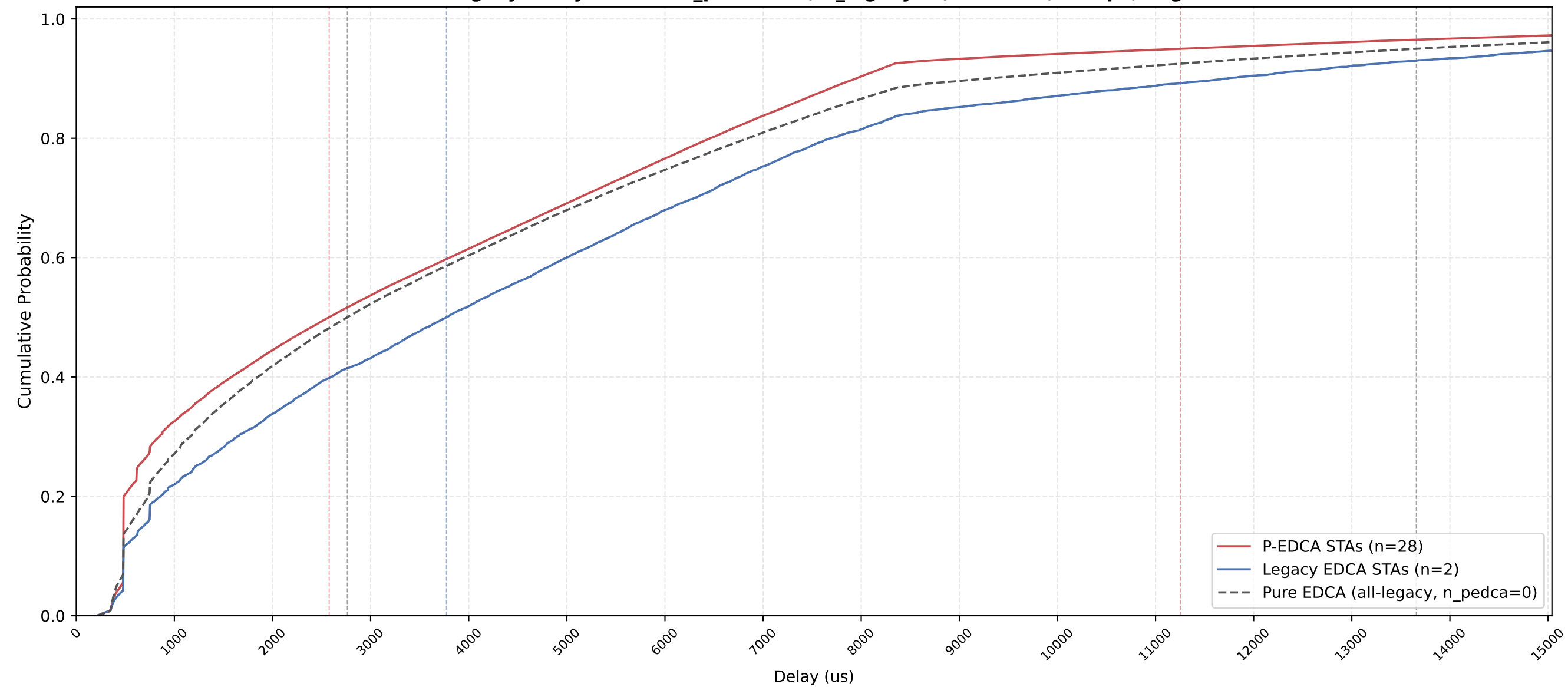
P-EDCA vs Legacy Delay CDF — n_pedca=28, n_legacy=2, nSta=30, 1Mbps, avg of 10 runs
