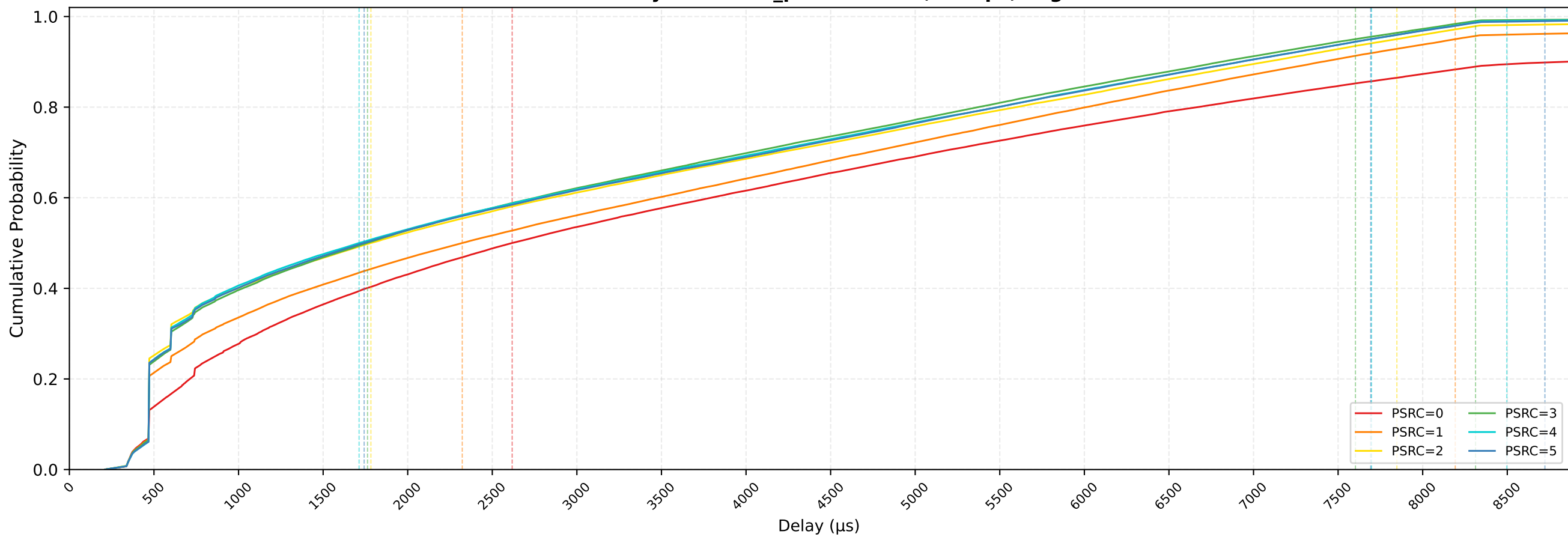
P-EDCA STAs Delay CDF — n_pedca=10/30, 1Mbps, avg of 10 runs
