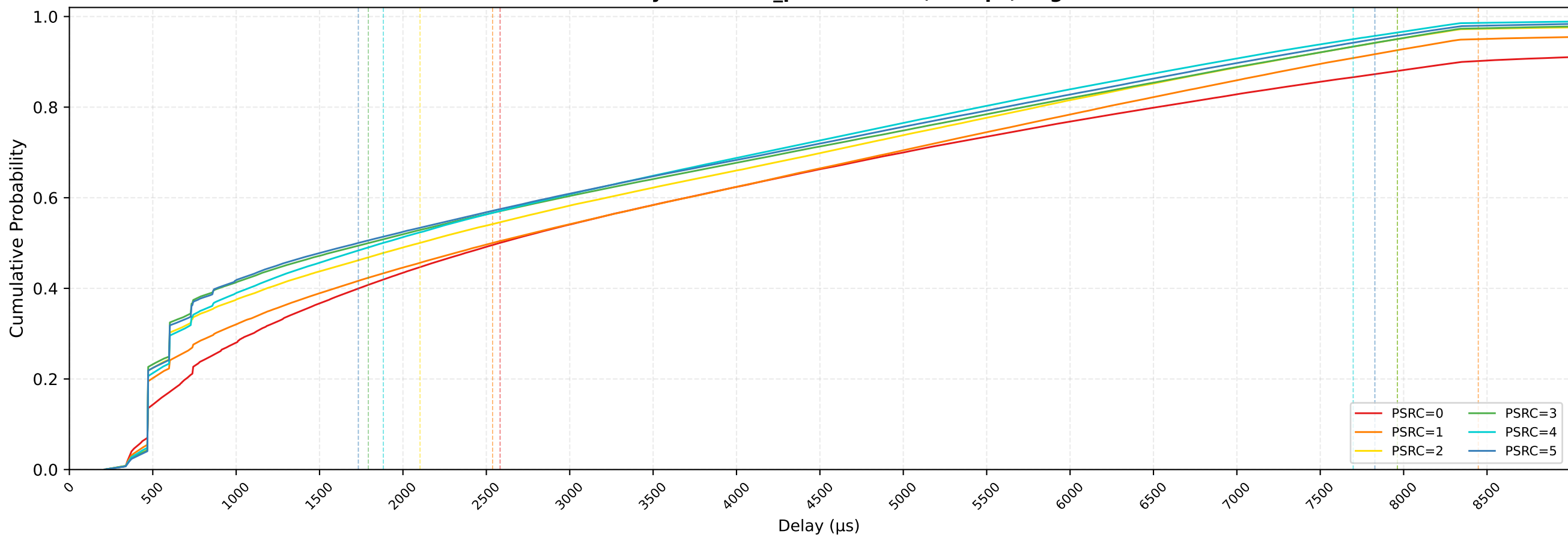
P-EDCA STAs Delay CDF — n_pedca=30/30, 1Mbps, avg of 10 runs
