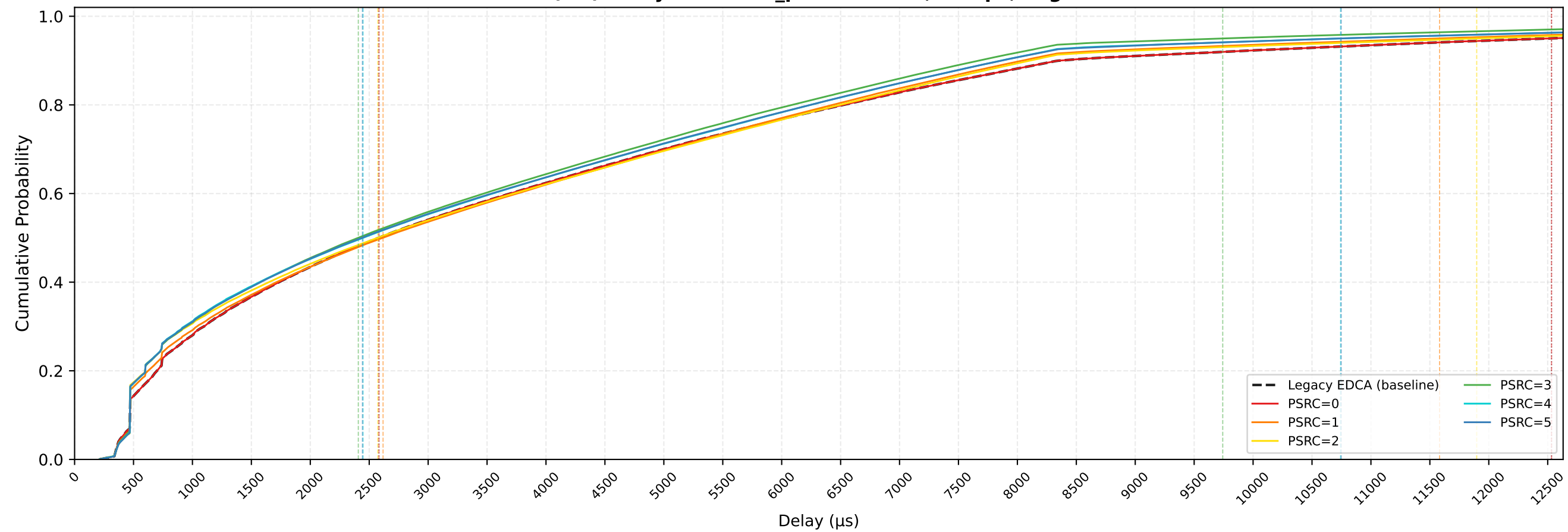
All STAs (VO) Delay CDF — n_pedca=10/30, 1Mbps, avg of 10 runs
