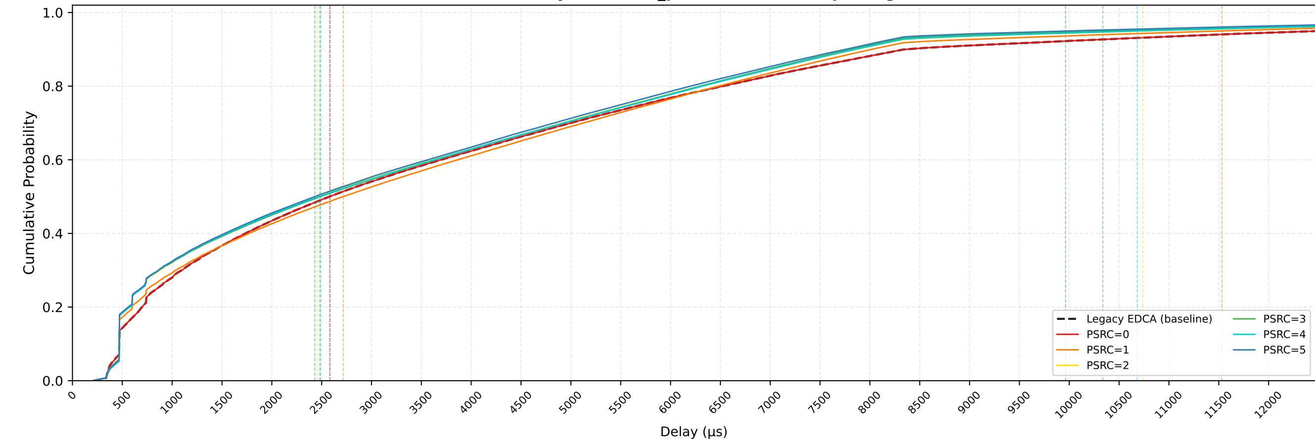
All STAs (VO) Delay CDF — n_pedca=15/30, 1Mbps, avg of 10 runs
