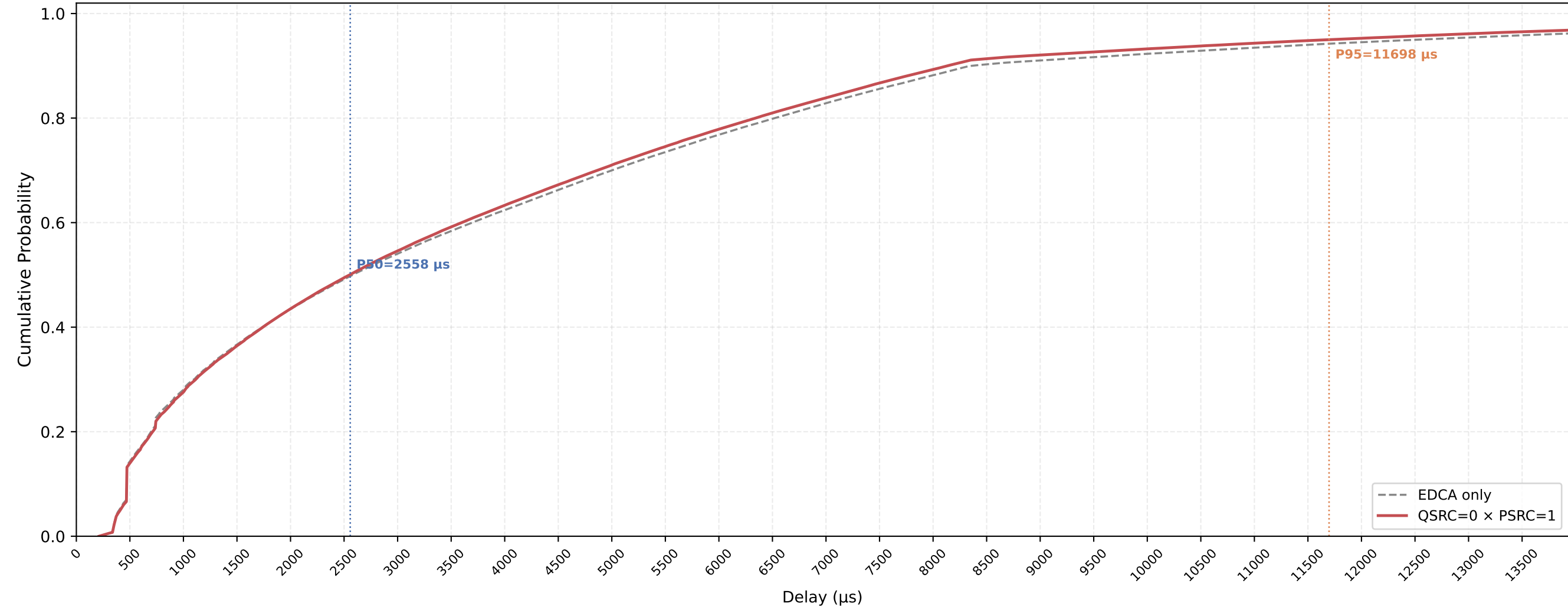
Legacy STA VO Delay CDF — QSRC=0 × PSRC=1 nSta=30, nPedca=5, 1Mbps, avg of 10 runs
