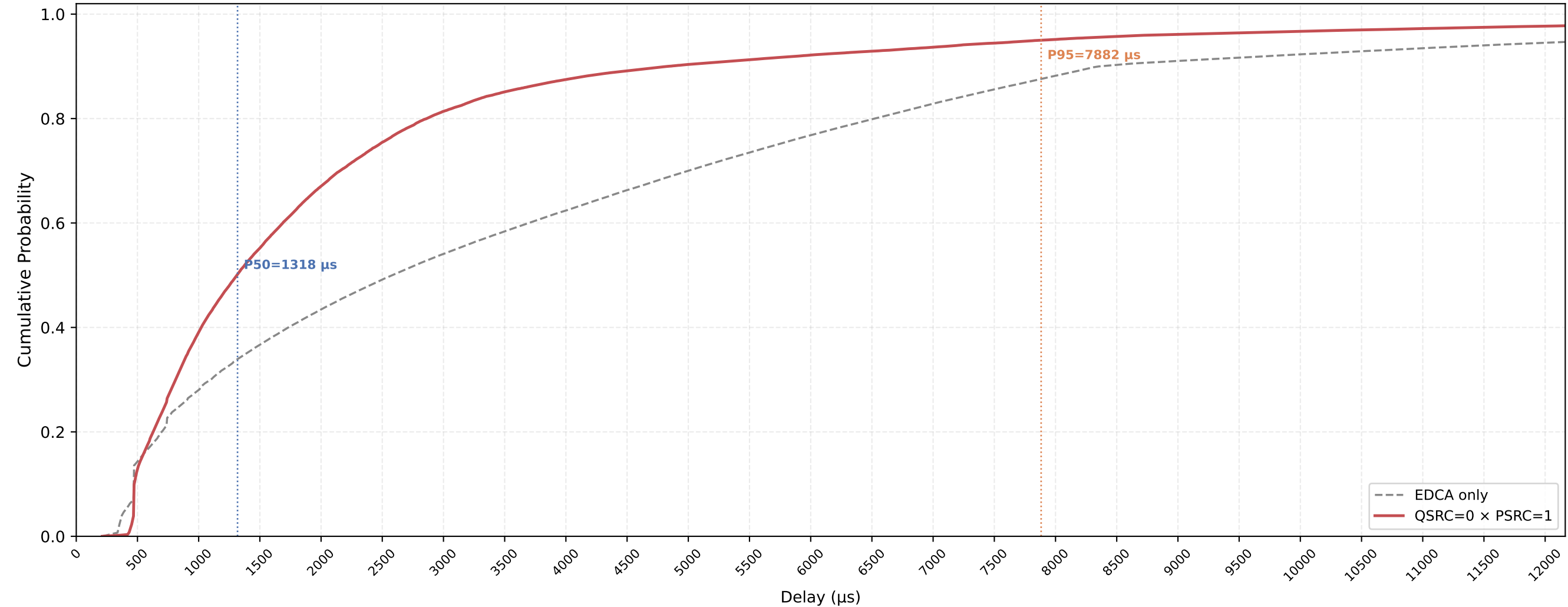
P-EDCA STA VO Delay CDF — QSRC=0 × PSRC=1 nSta=30, nPedca=5, 1Mbps, avg of 10 runs
