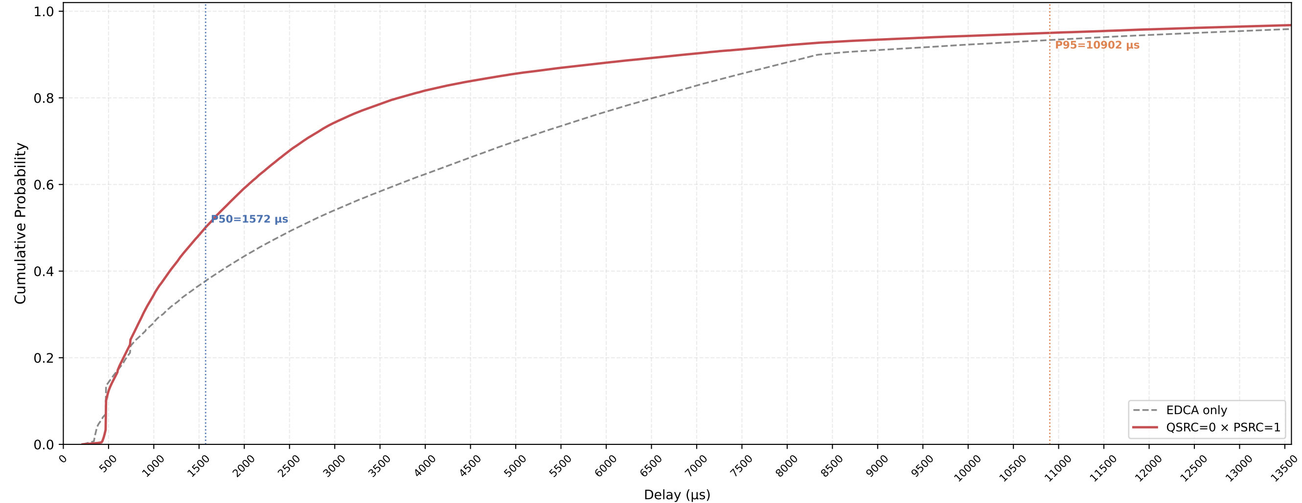
P-EDCA STA VO Delay CDF — QSRC=0 × PSRC=1 nSta=30, nPedca=15, 1Mbps, avg of 10 runs
