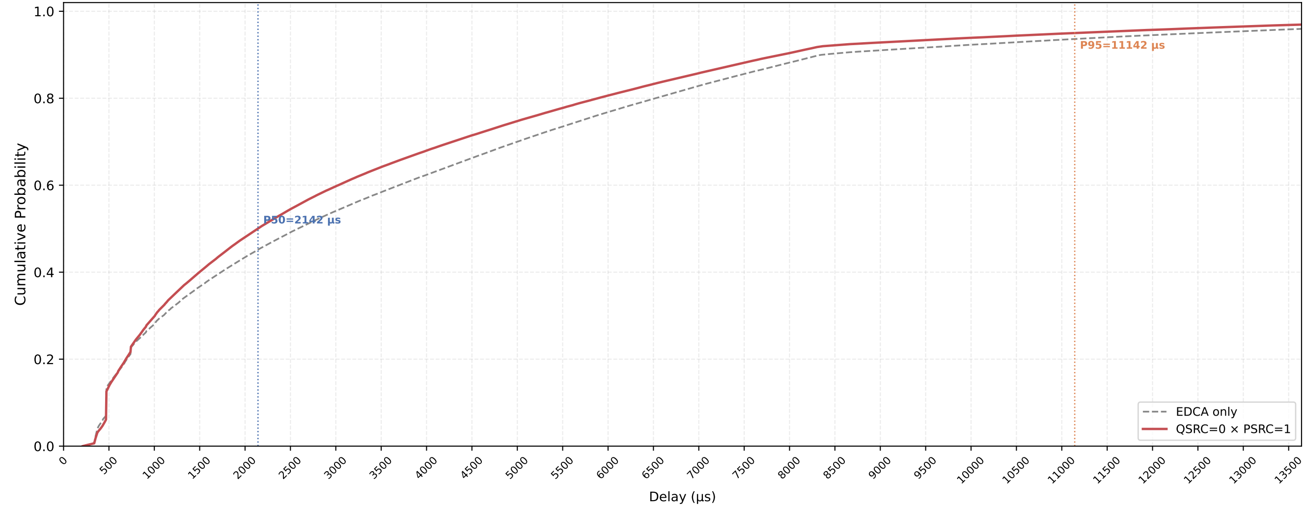
VO (all STAs) Delay CDF — QSRC=0 × PSRC=1 nSta=30, nPedca=5, 1Mbps, avg of 10 runs
