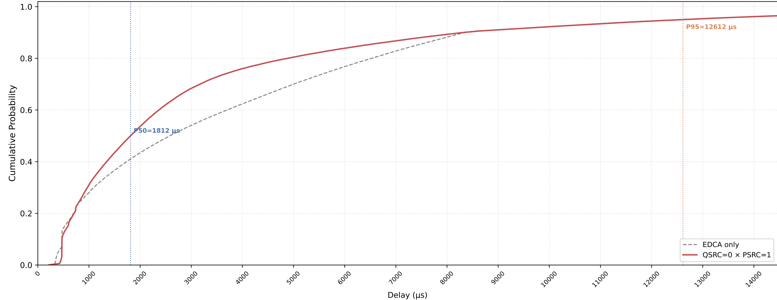
VO (all STAs) Delay CDF — QSRC=0 × PSRC=1 nSta=30, nPedca=30, 1Mbps, avg of 10 runs
