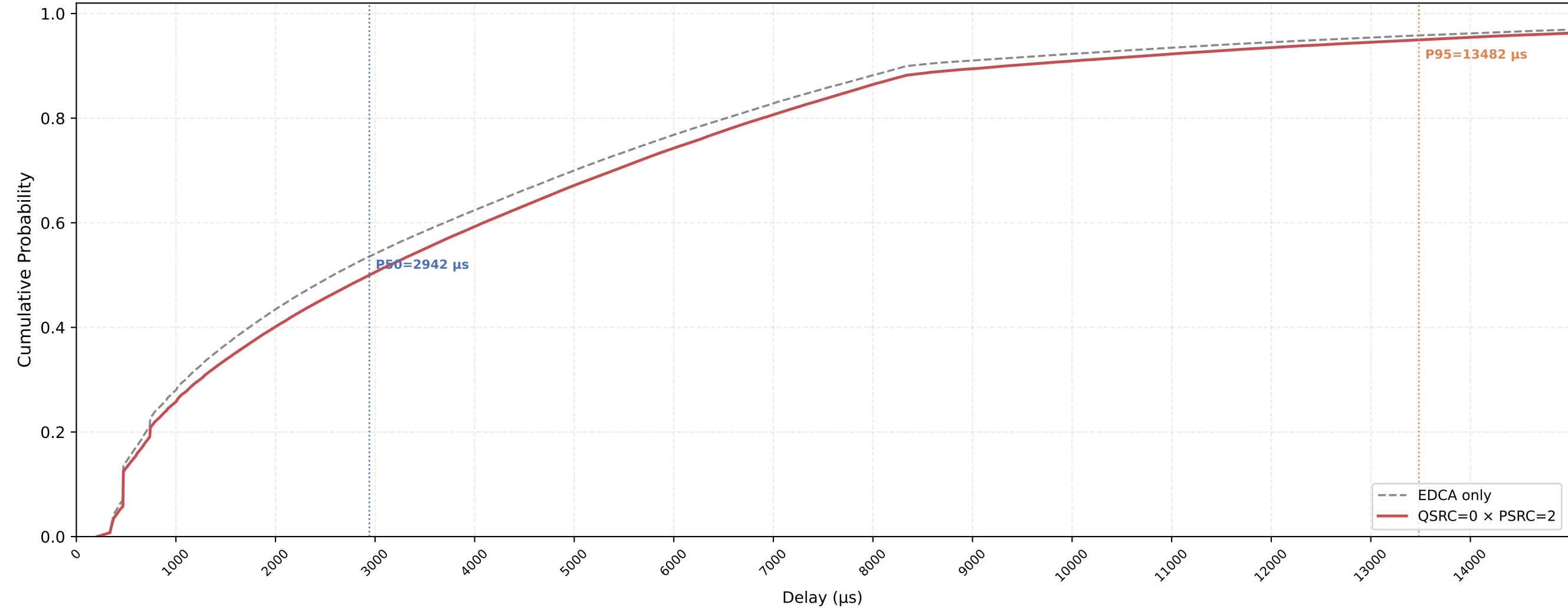
Legacy STA VO Delay CDF — QSRC=0 × PSRC=2 nSta=30, nPedca=5, 1Mbps, avg of 10 runs
