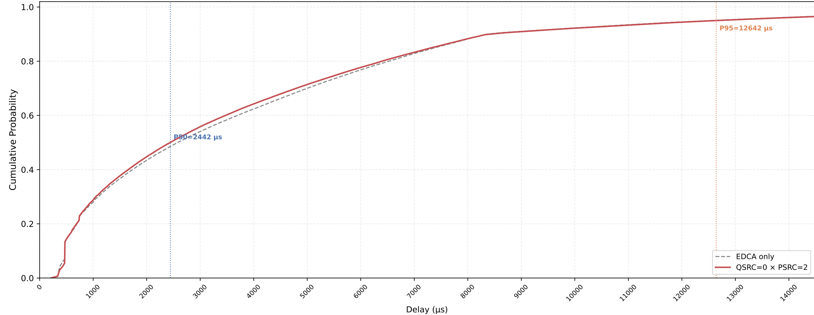
VO (all STAs) Delay CDF — QSRC=0 × PSRC=2 nSta=30, nPedca=5, 1Mbps, avg of 10 runs
