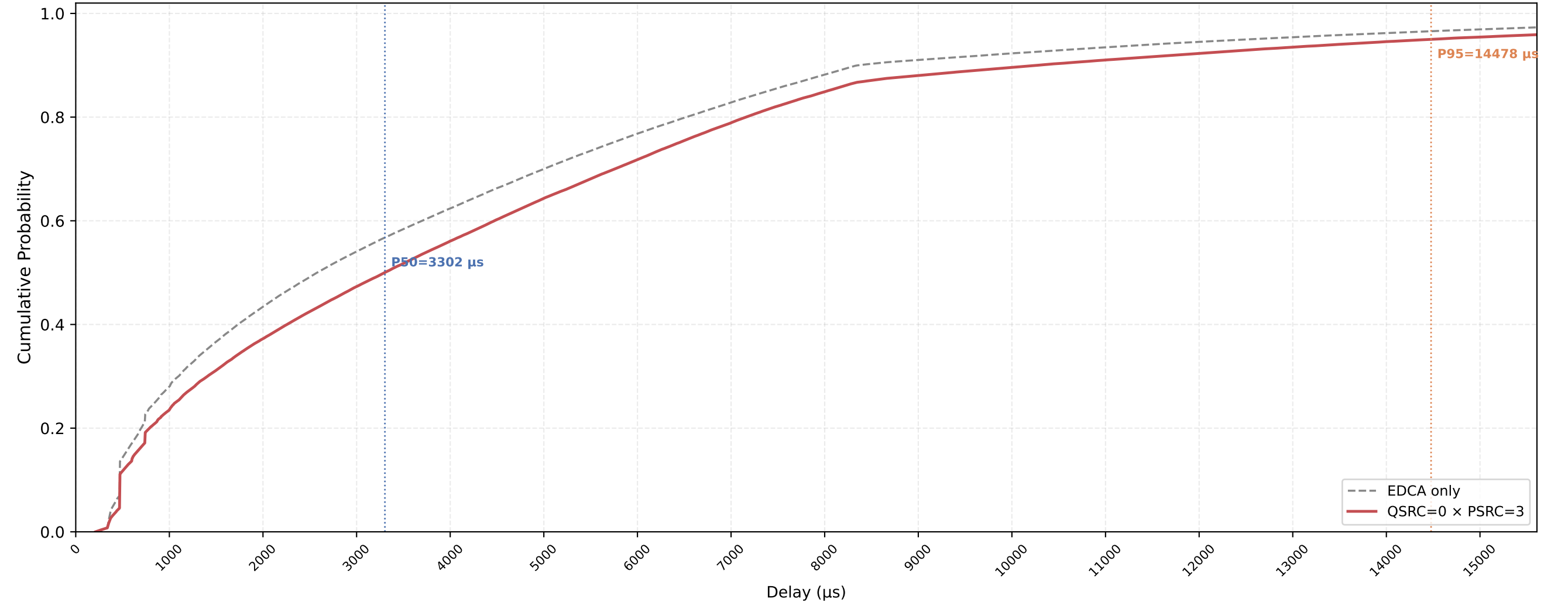
Legacy STA VO Delay CDF — QSRC=0 × PSRC=3 nSta=30, nPedca=15, 1Mbps, avg of 10 runs
