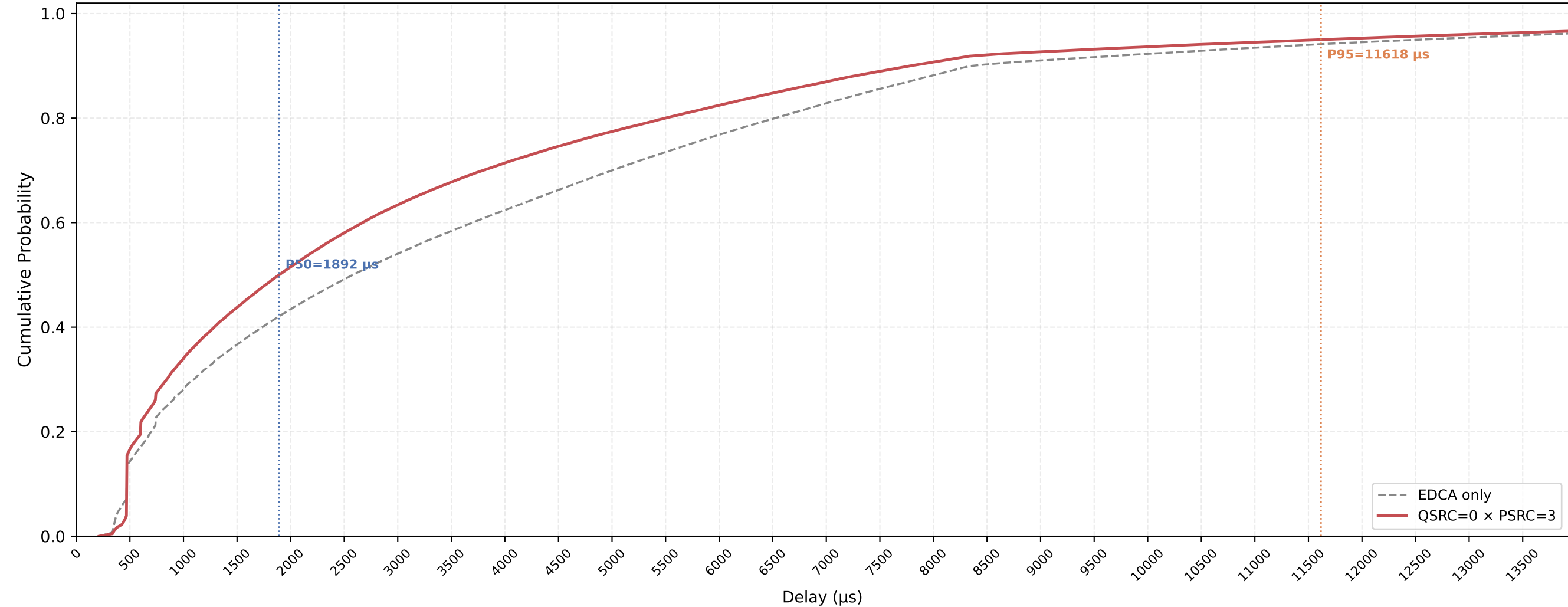
VO (all STAs) Delay CDF — QSRC=0 × PSRC=3 nSta=30, nPedca=15, 1Mbps, avg of 10 runs
