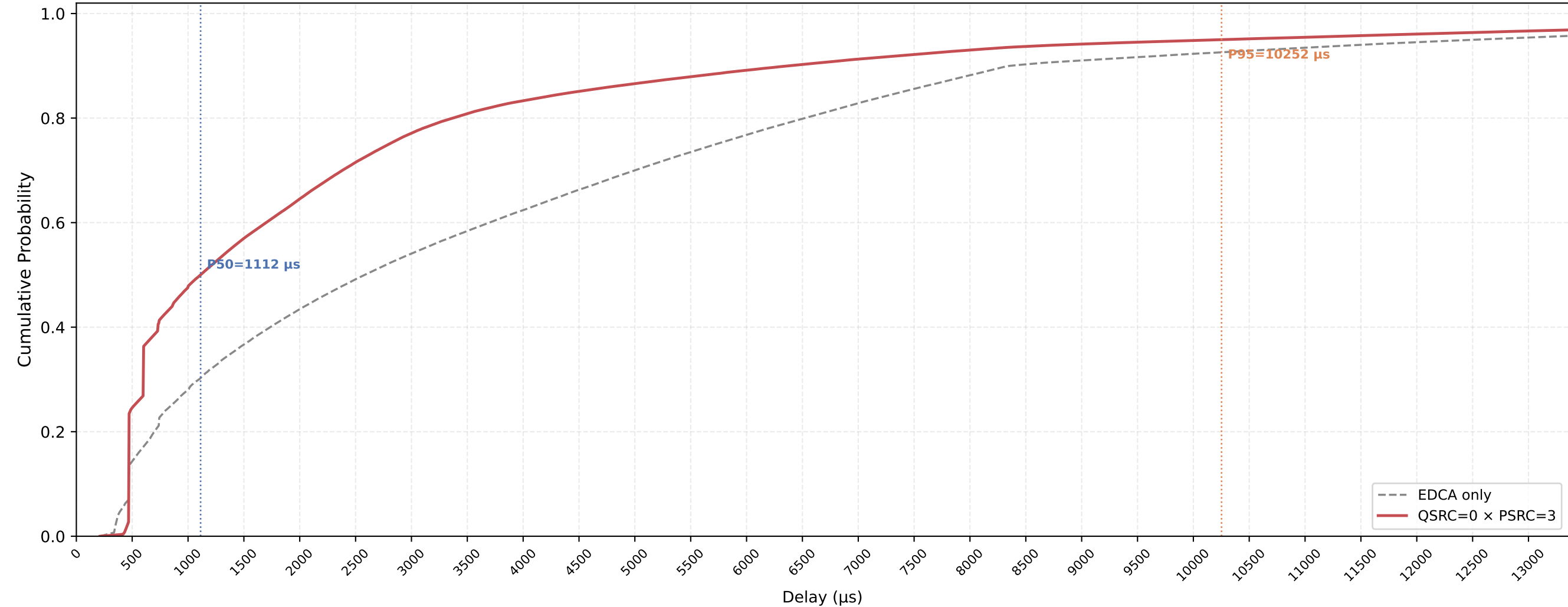
VO (all STAs) Delay CDF — QSRC=0 × PSRC=3 nSta=30, nPedca=30, 1Mbps, avg of 10 runs
