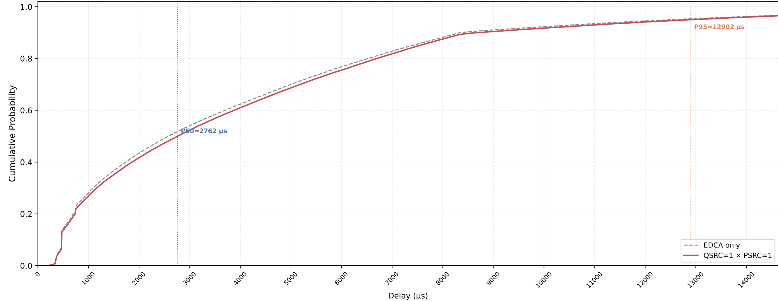
Legacy STA VO Delay CDF — QSRC=1 × PSRC=1 nSta=30, nPedca=5, 1Mbps, avg of 10 runs
