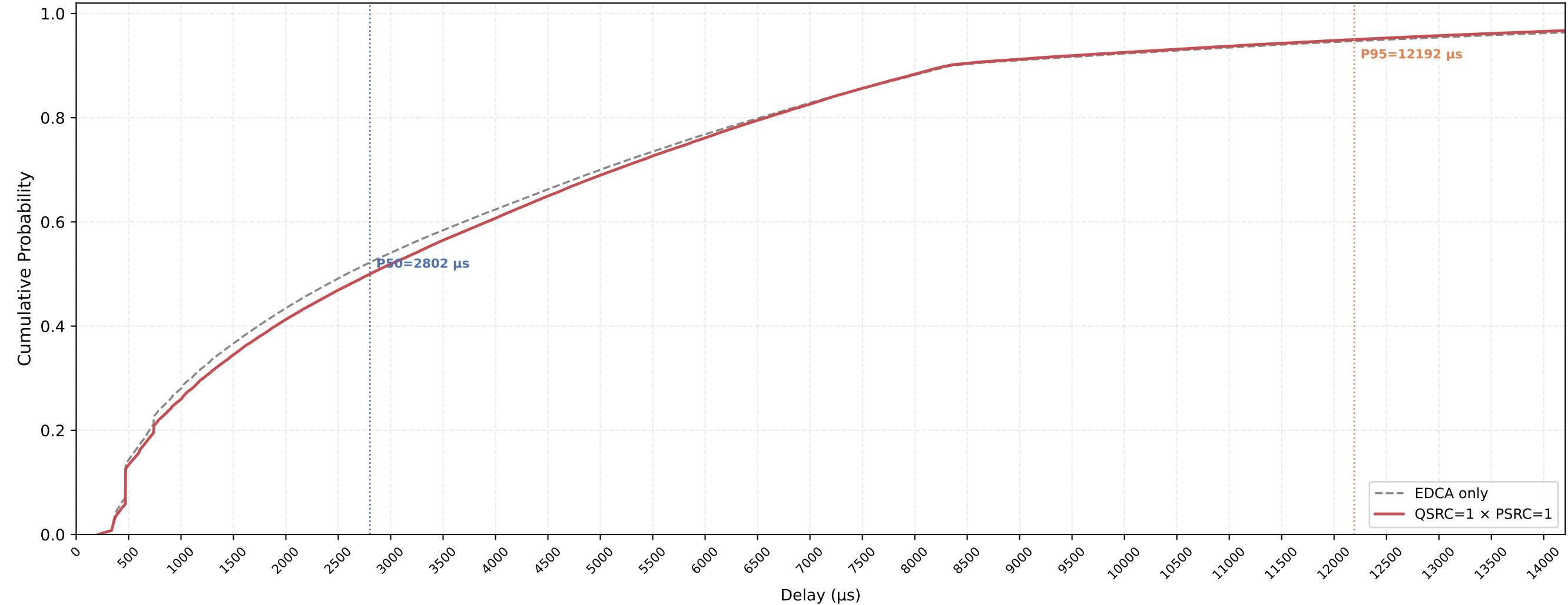
Legacy STA VO Delay CDF — QSRC=1 × PSRC=1 nSta=30, nPedca=15, 1Mbps, avg of 10 runs
