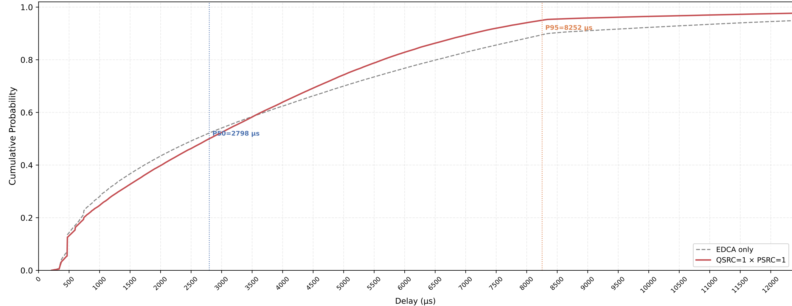
P-EDCA STA VO Delay CDF — QSRC=1 × PSRC=1 nSta=30, nPedca=15, 1Mbps, avg of 10 runs
