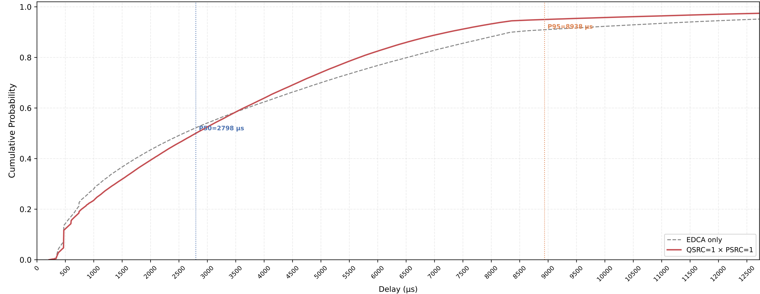
P-EDCA STA VO Delay CDF — QSRC=1 × PSRC=1 nSta=30, nPedca=30, 1Mbps, avg of 10 runs
