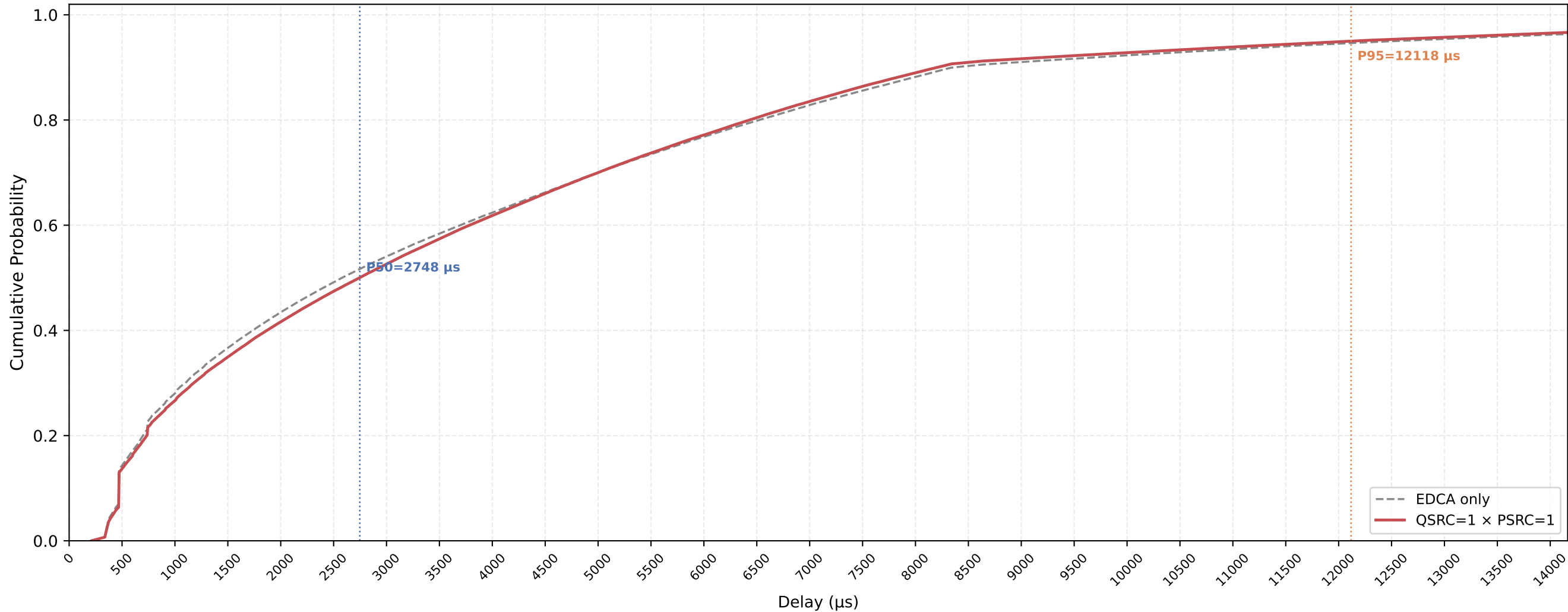
VO (all STAs) Delay CDF — QSRC=1 × PSRC=1 nSta=30, nPedca=5, 1Mbps, avg of 10 runs
