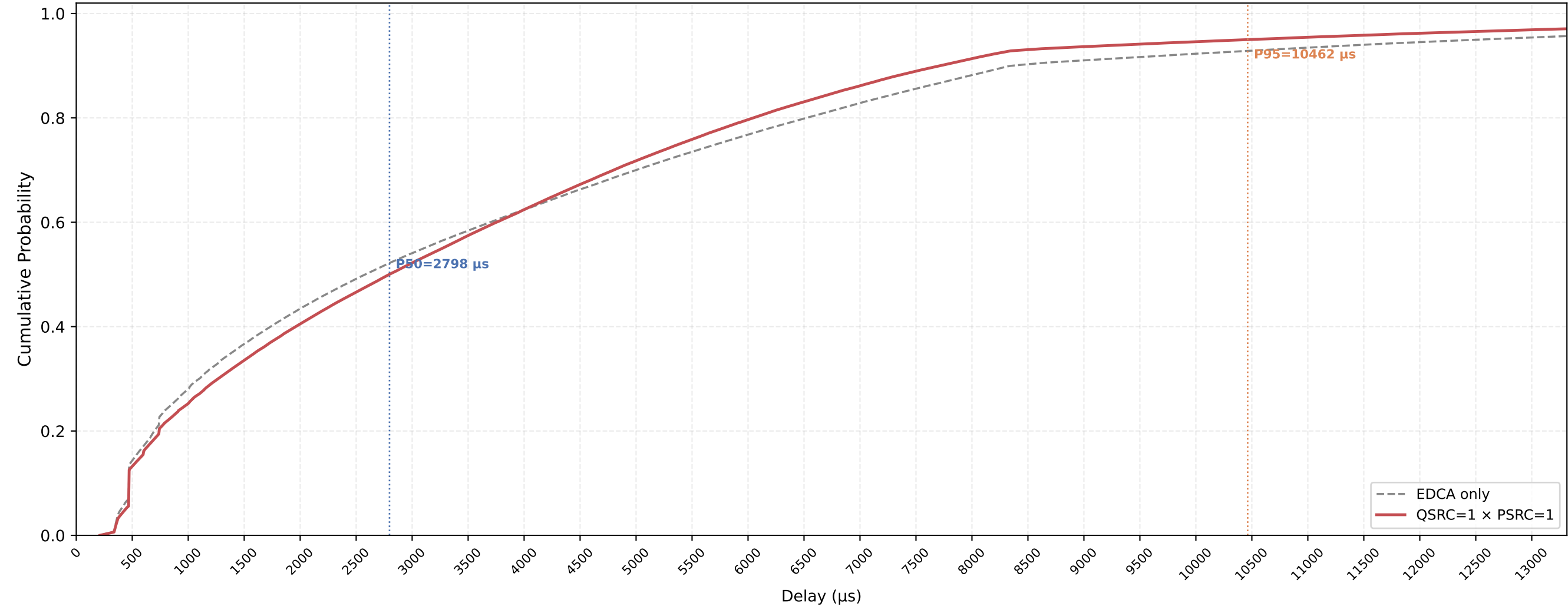
VO (all STAs) Delay CDF — QSRC=1 × PSRC=1 nSta=30, nPedca=15, 1Mbps, avg of 10 runs
