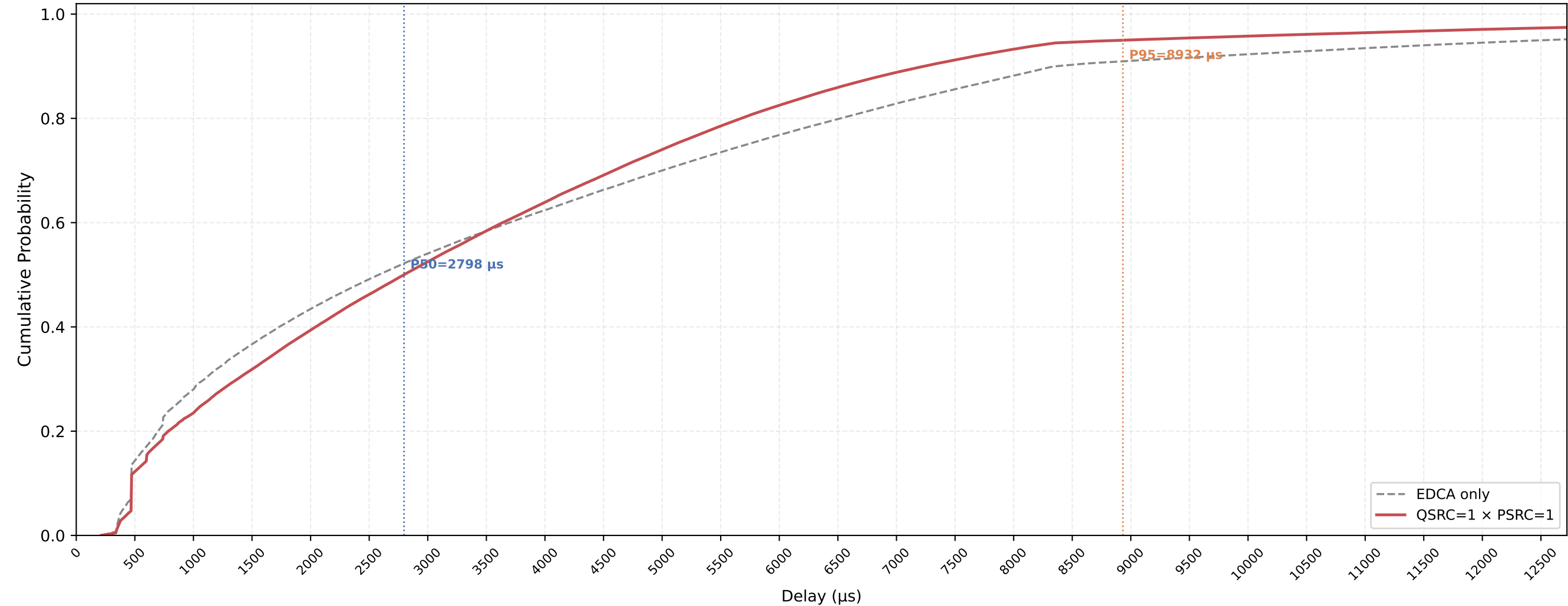
VO (all STAs) Delay CDF — QSRC=1 × PSRC=1 nSta=30, nPedca=30, 1Mbps, avg of 10 runs
