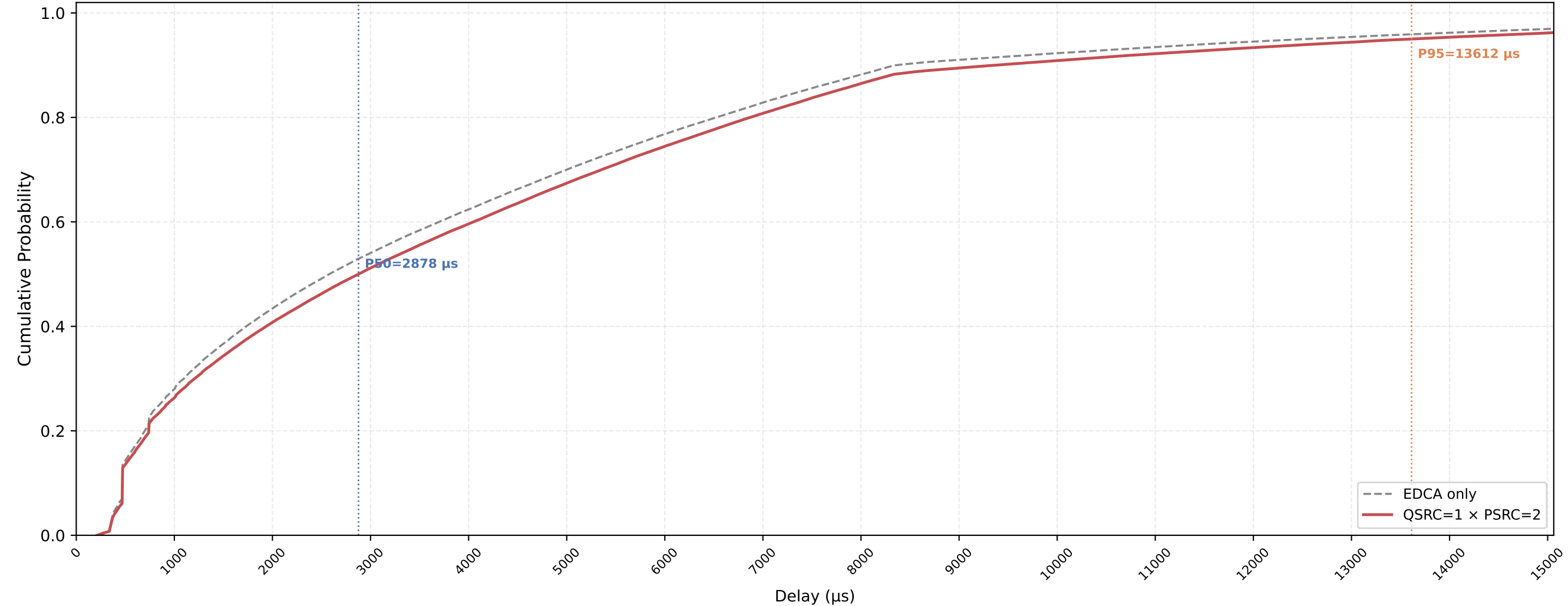
Legacy STA VO Delay CDF — QSRC=1 × PSRC=2 nSta=30, nPedca=5, 1Mbps, avg of 10 runs
