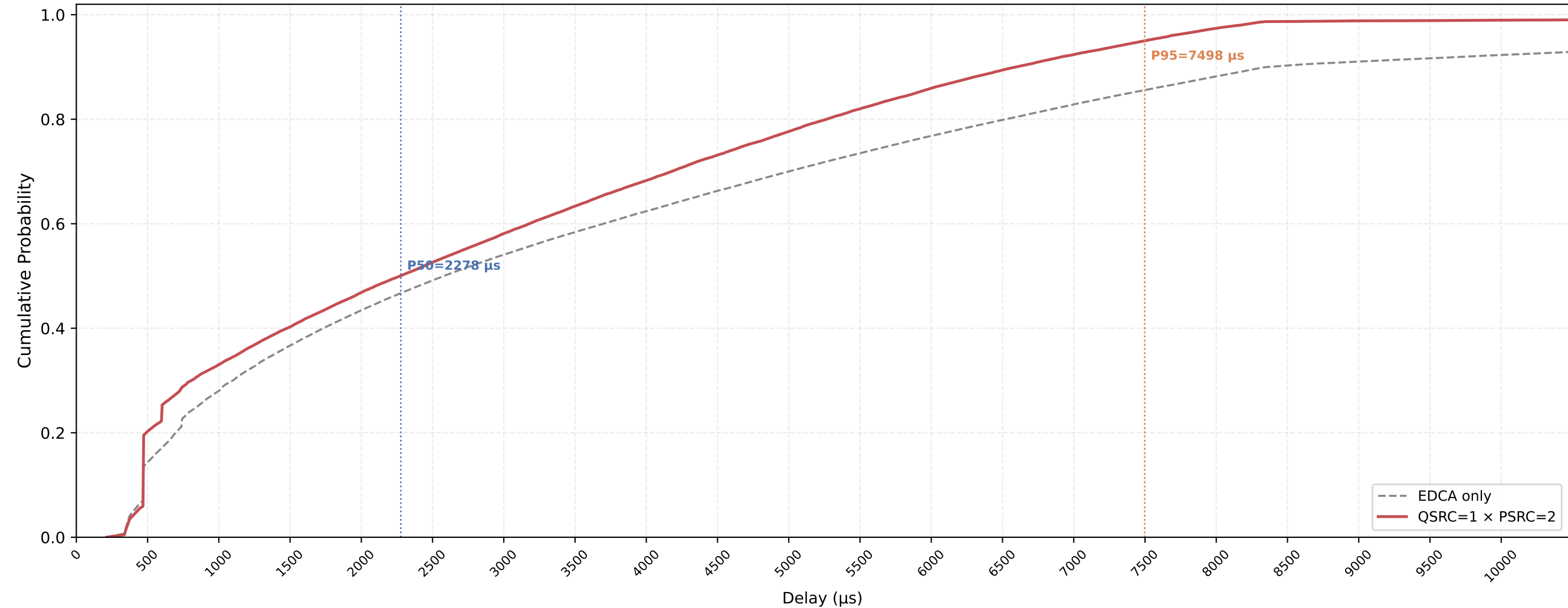
P-EDCA STA VO Delay CDF — QSRC=1 × PSRC=2 nSta=30, nPedca=5, 1Mbps, avg of 10 runs
