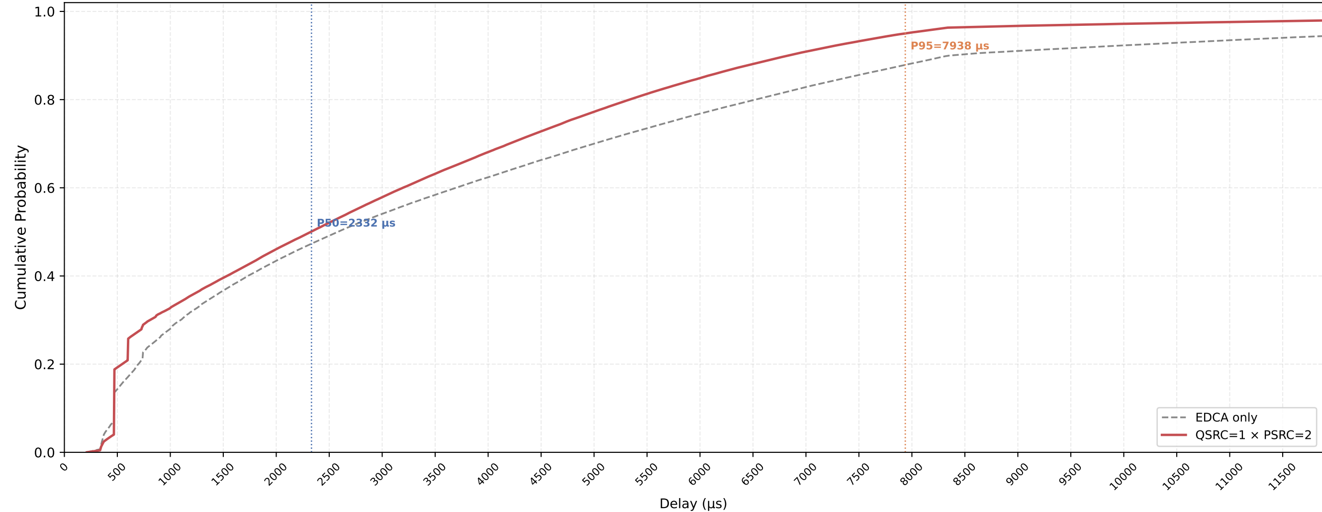
VO (all STAs) Delay CDF — QSRC=1 × PSRC=2 nSta=30, nPedca=30, 1Mbps, avg of 10 runs
