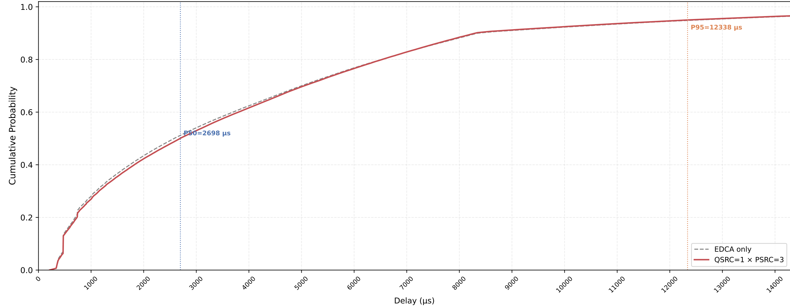
Legacy STA VO Delay CDF — QSRC=1 × PSRC=3 nSta=30, nPedca=5, 1Mbps, avg of 10 runs
