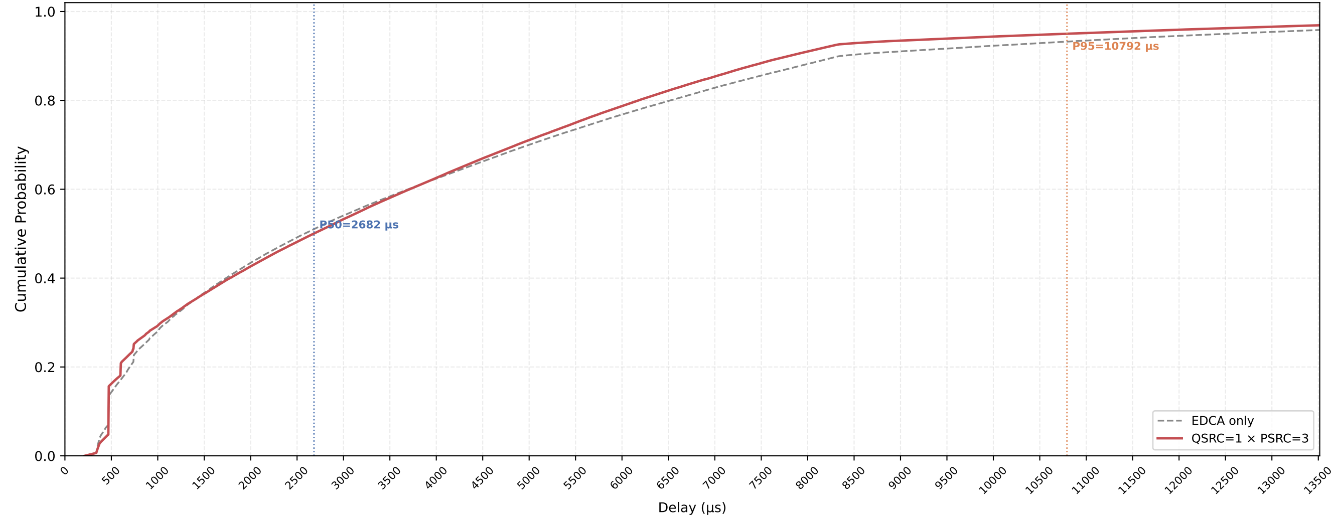
VO (all STAs) Delay CDF — QSRC=1 × PSRC=3 nSta=30, nPedca=15, 1Mbps, avg of 10 runs
