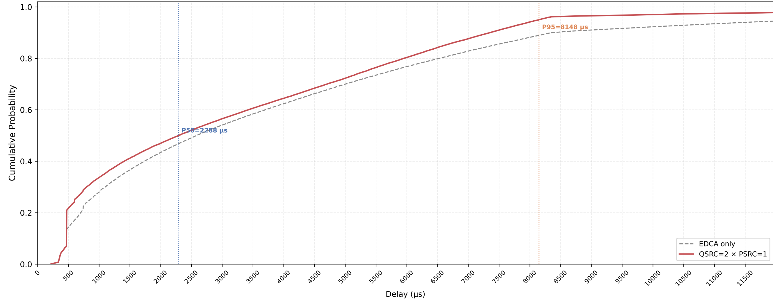
P-EDCA STA VO Delay CDF — QSRC=2 × PSRC=1 nSta=30, nPedca=5, 1Mbps, avg of 10 runs
