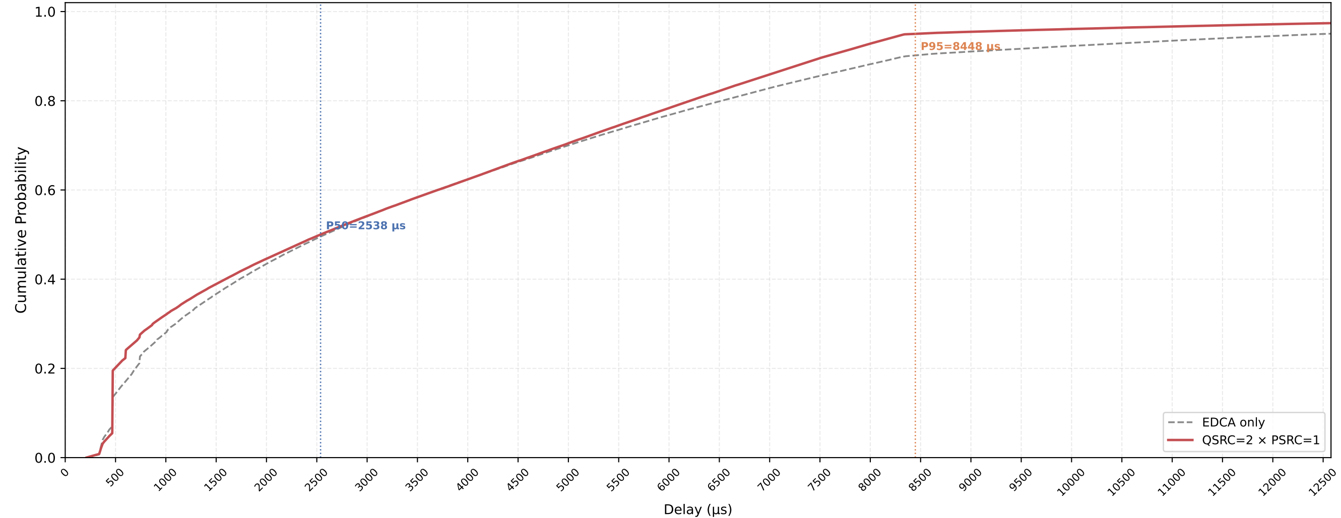
P-EDCA STA VO Delay CDF — QSRC=2 × PSRC=1 nSta=30, nPedca=30, 1Mbps, avg of 10 runs
