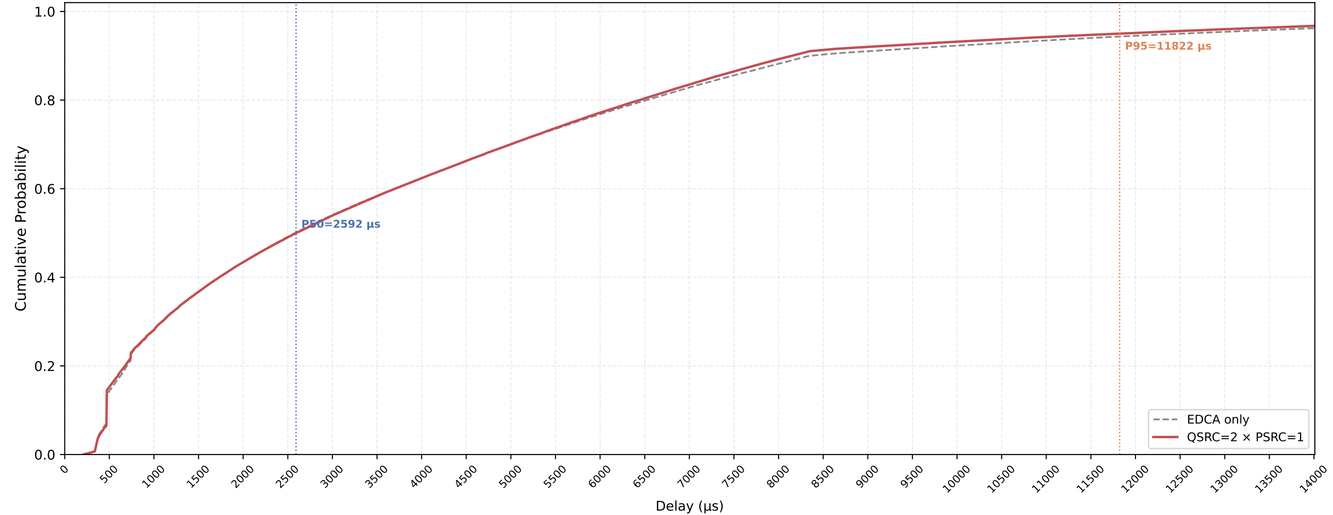
VO (all STAs) Delay CDF — QSRC=2 × PSRC=1 nSta=30, nPedca=5, 1Mbps, avg of 10 runs
