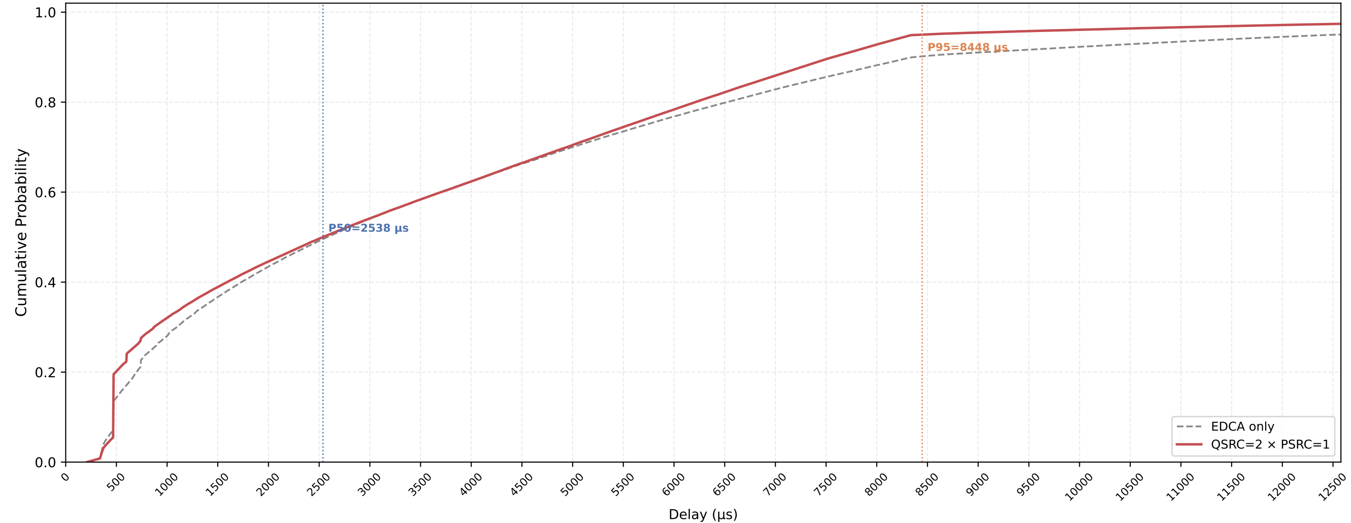
VO (all STAs) Delay CDF — QSRC=2 × PSRC=1 nSta=30, nPedca=30, 1Mbps, avg of 10 runs
