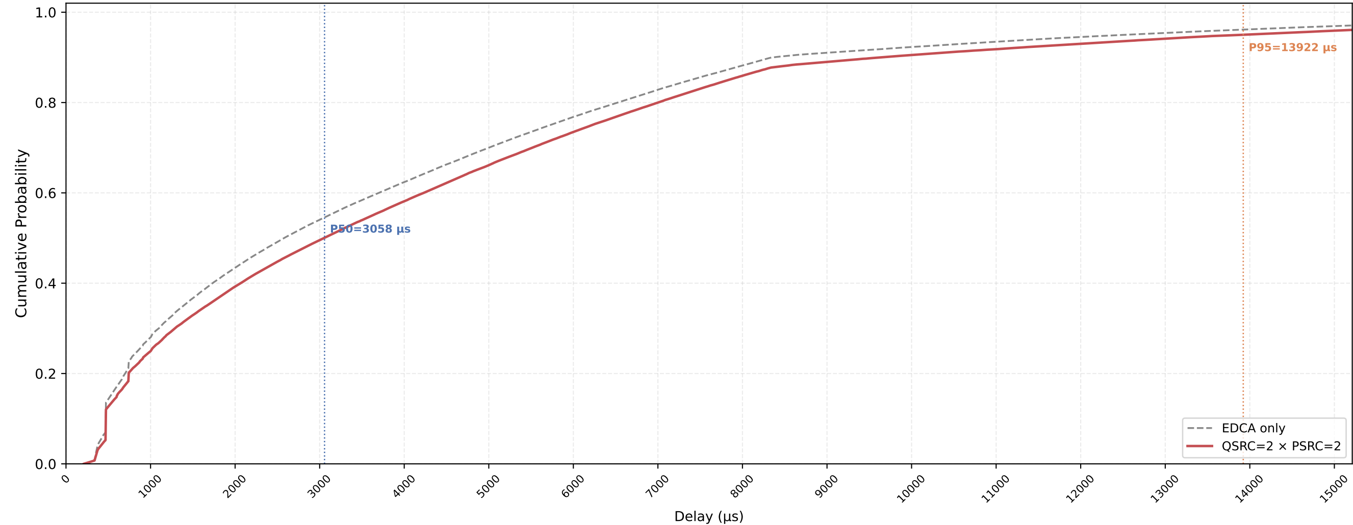
Legacy STA VO Delay CDF — QSRC=2 × PSRC=2 nSta=30, nPedca=15, 1Mbps, avg of 10 runs
