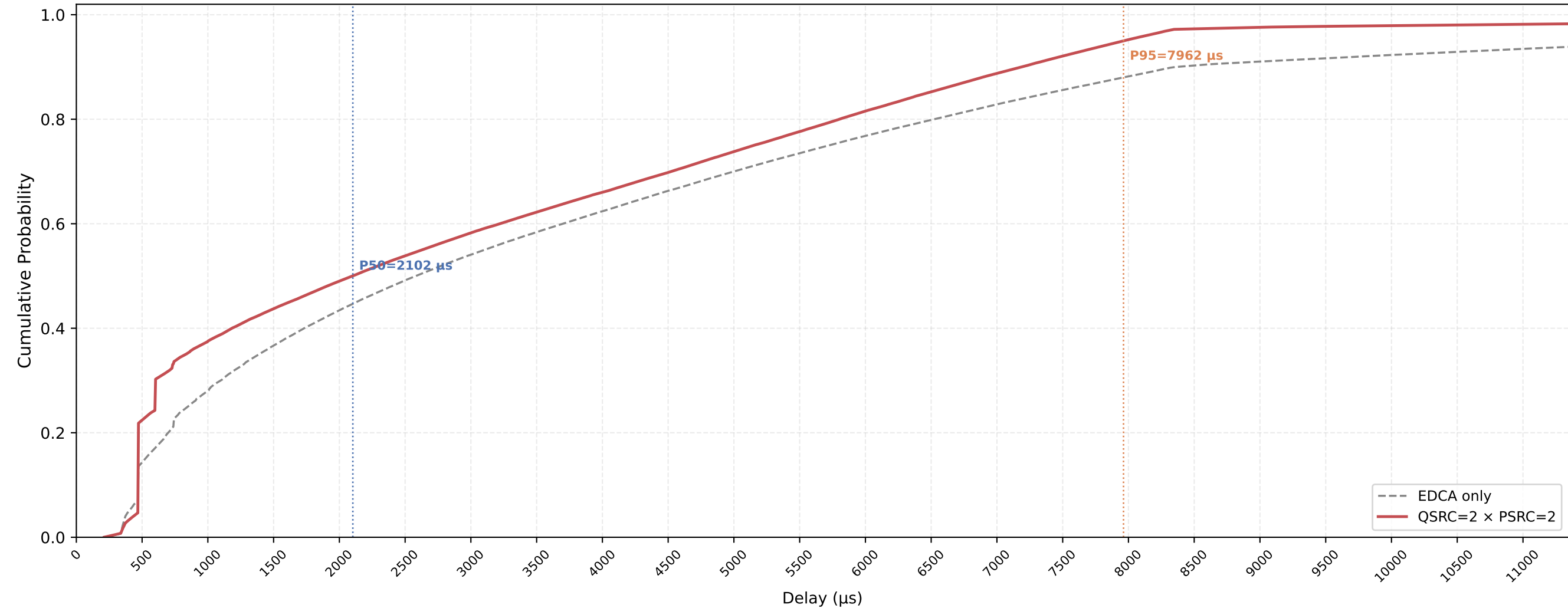
P-EDCA STA VO Delay CDF — QSRC=2 × PSRC=2 nSta=30, nPedca=30, 1Mbps, avg of 10 runs
