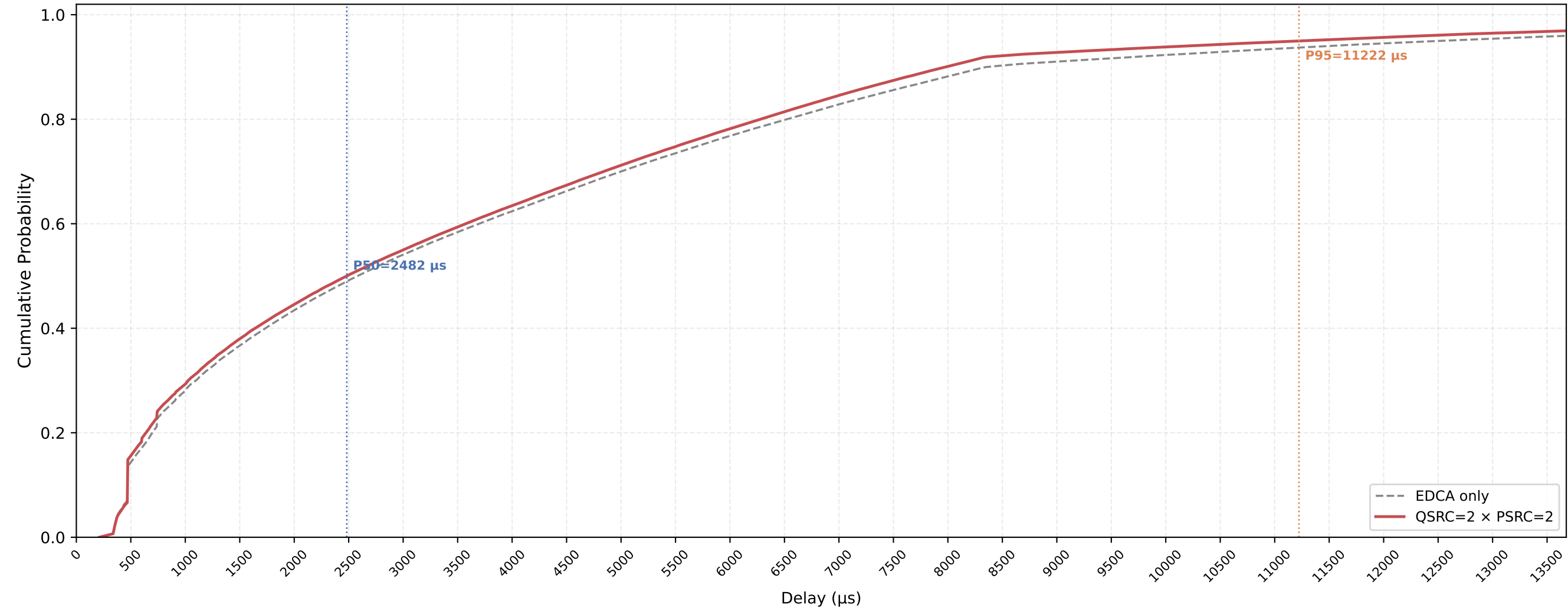
VO (all STAs) Delay CDF — QSRC=2 × PSRC=2 nSta=30, nPedca=5, 1Mbps, avg of 10 runs
