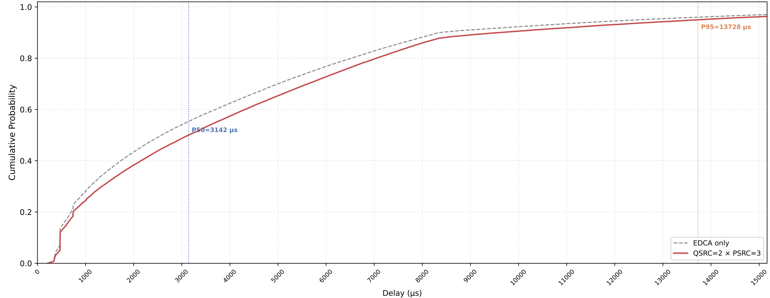
Legacy STA VO Delay CDF — QSRC=2 × PSRC=3 nSta=30, nPedca=15, 1Mbps, avg of 10 runs
