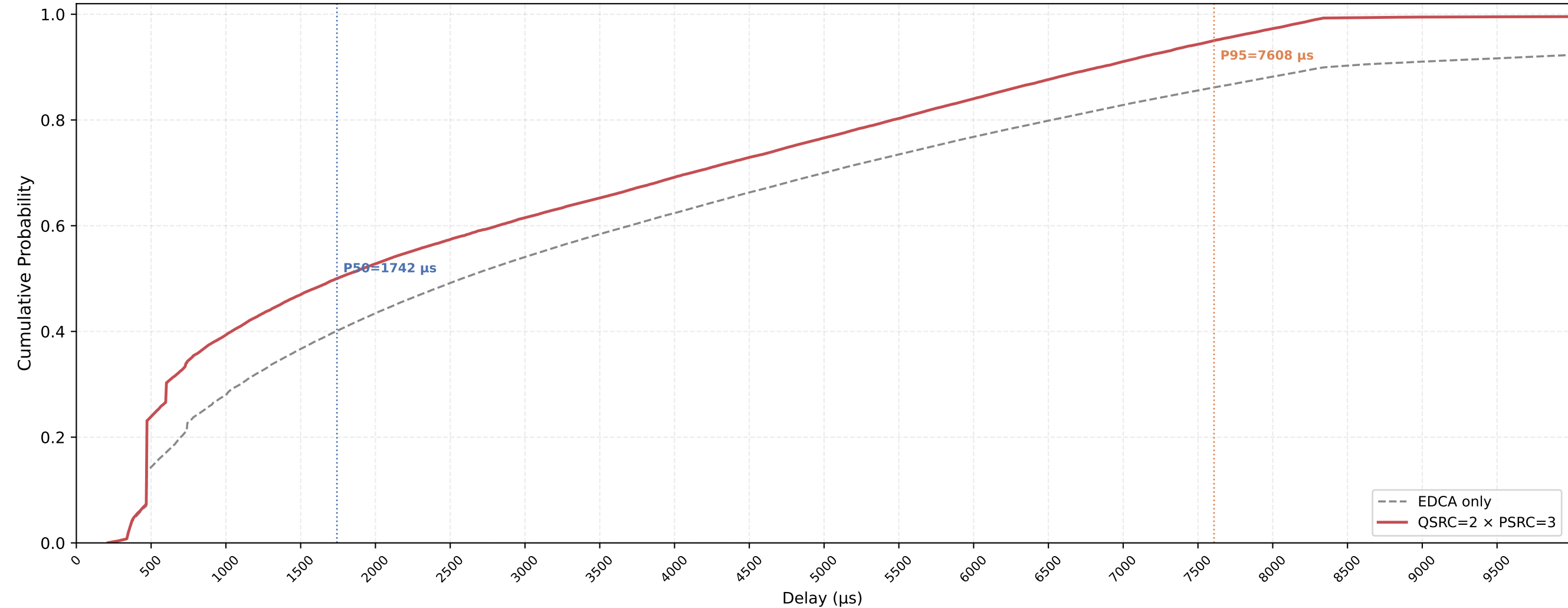
P-EDCA STA VO Delay CDF — QSRC=2 × PSRC=3 nSta=30, nPedca=5, 1Mbps, avg of 10 runs
