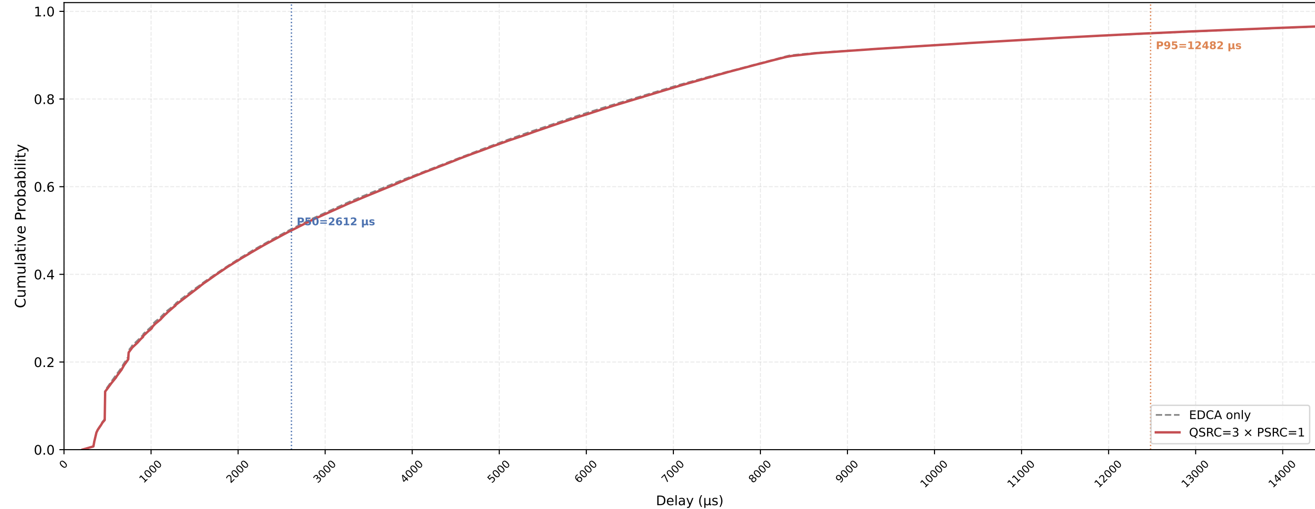
Legacy STA VO Delay CDF — QSRC=3 × PSRC=1 nSta=30, nPedca=5, 1Mbps, avg of 10 runs
