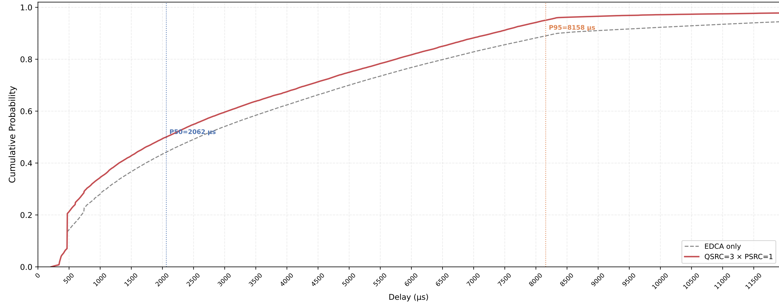
P-EDCA STA VO Delay CDF — QSRC=3 × PSRC=1 nSta=30, nPedca=5, 1Mbps, avg of 10 runs
