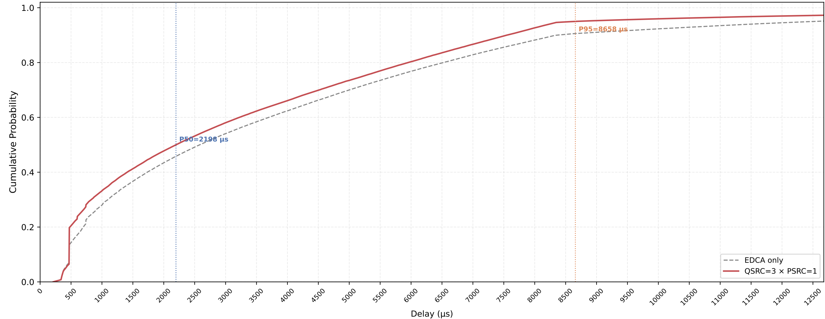
P-EDCA STA VO Delay CDF — QSRC=3 × PSRC=1 nSta=30, nPedca=15, 1Mbps, avg of 10 runs
