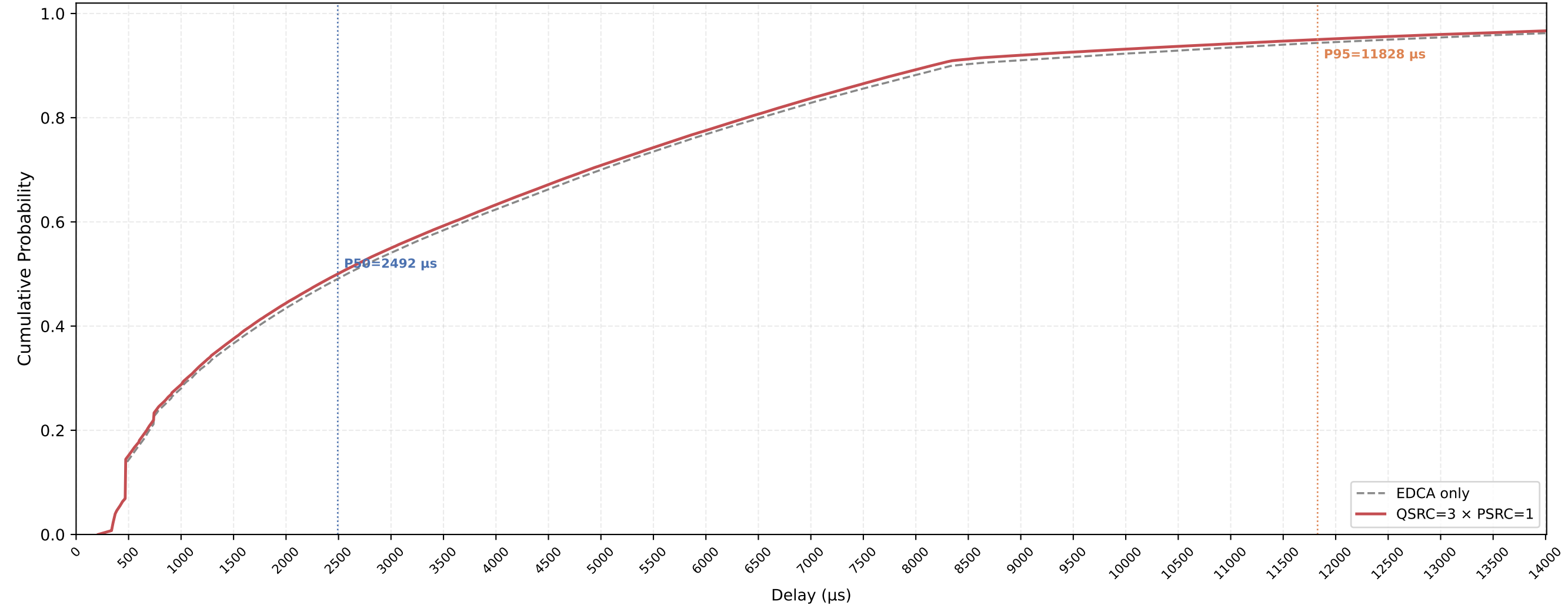
VO (all STAs) Delay CDF — QSRC=3 × PSRC=1 nSta=30, nPedca=5, 1Mbps, avg of 10 runs
