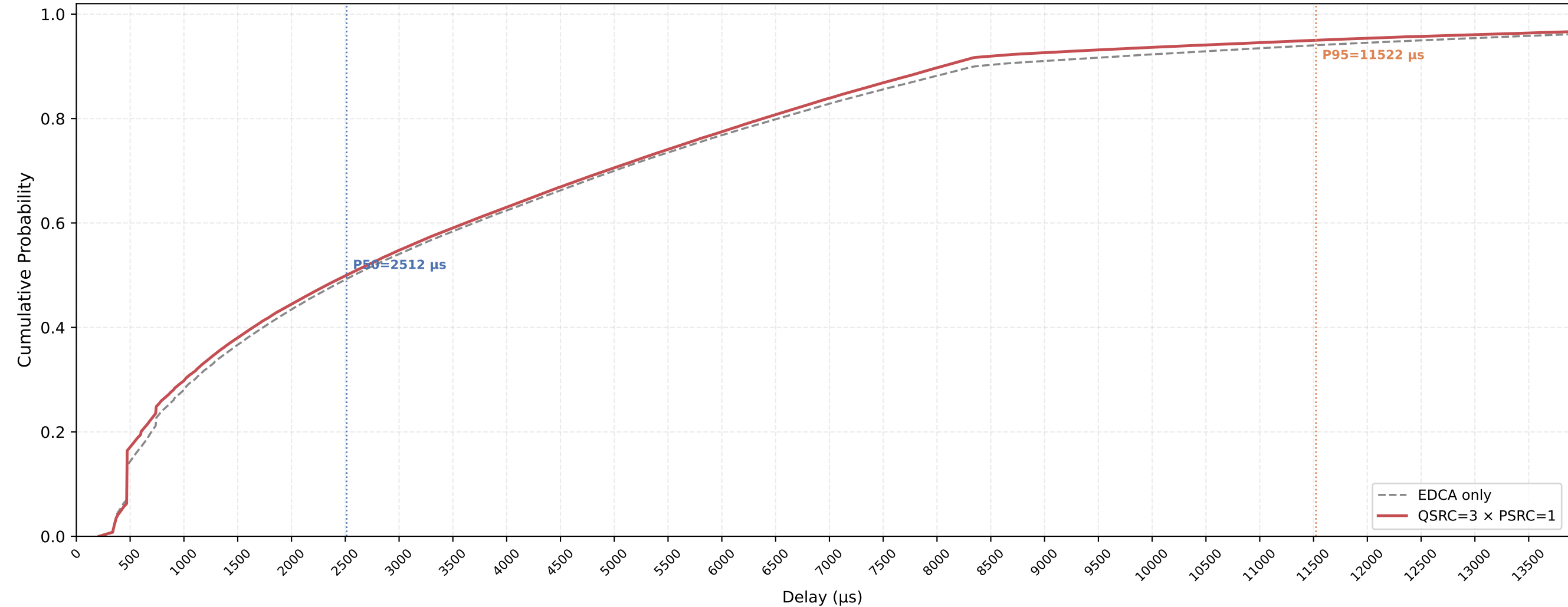
VO (all STAs) Delay CDF — QSRC=3 × PSRC=1 nSta=30, nPedca=15, 1Mbps, avg of 10 runs
