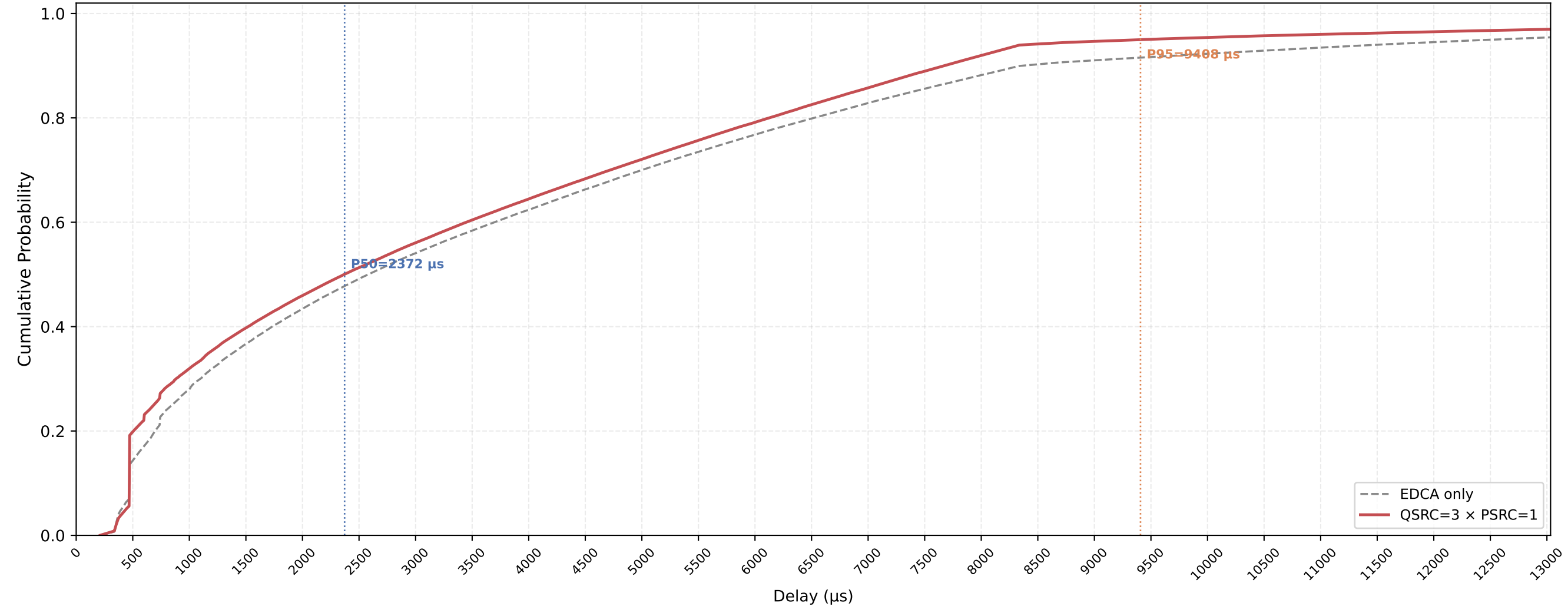
VO (all STAs) Delay CDF — QSRC=3 × PSRC=1 nSta=30, nPedca=30, 1Mbps, avg of 10 runs
