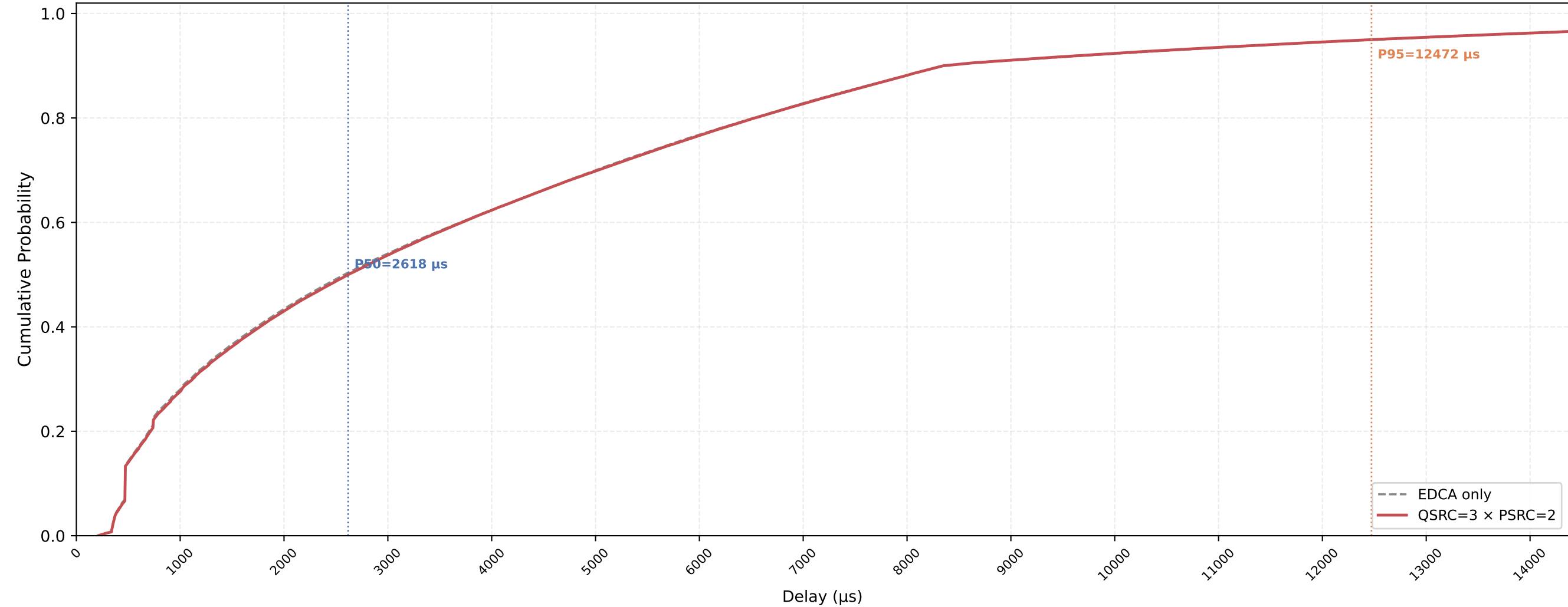
Legacy STA VO Delay CDF — QSRC=3 × PSRC=2 nSta=30, nPedca=5, 1Mbps, avg of 10 runs
