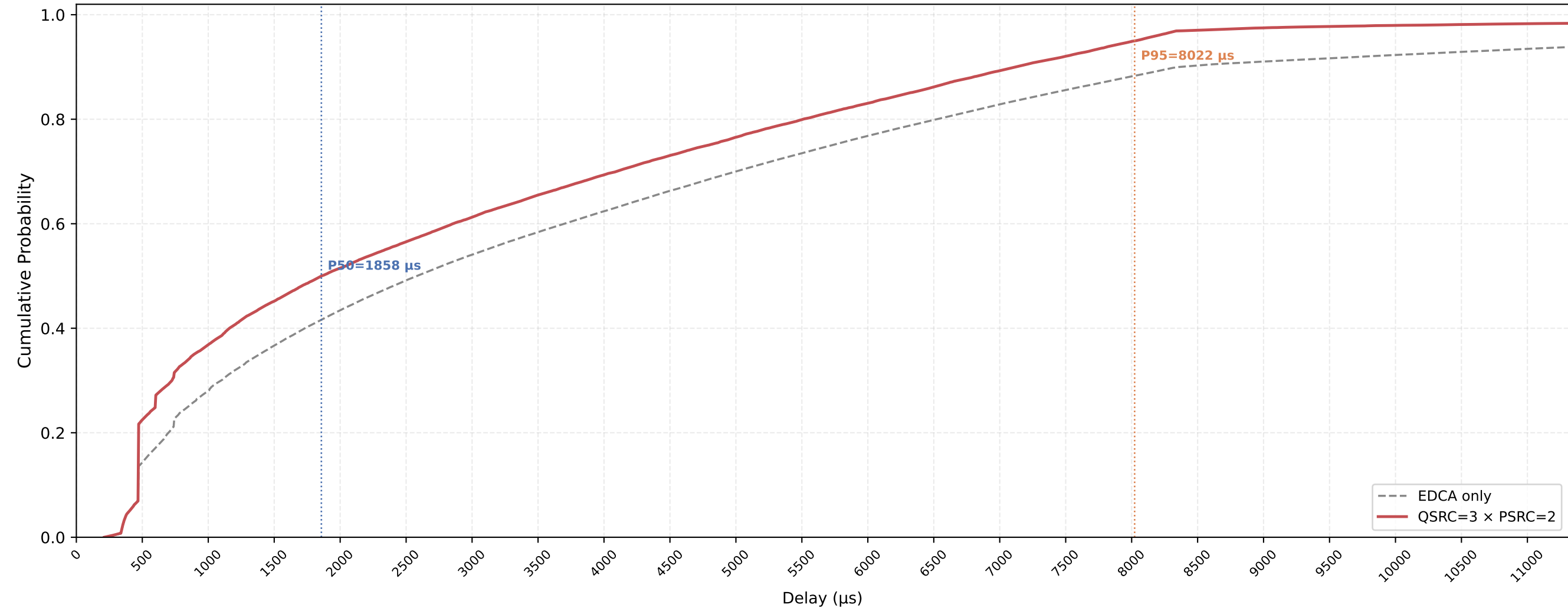
P-EDCA STA VO Delay CDF — QSRC=3 × PSRC=2 nSta=30, nPedca=5, 1Mbps, avg of 10 runs
