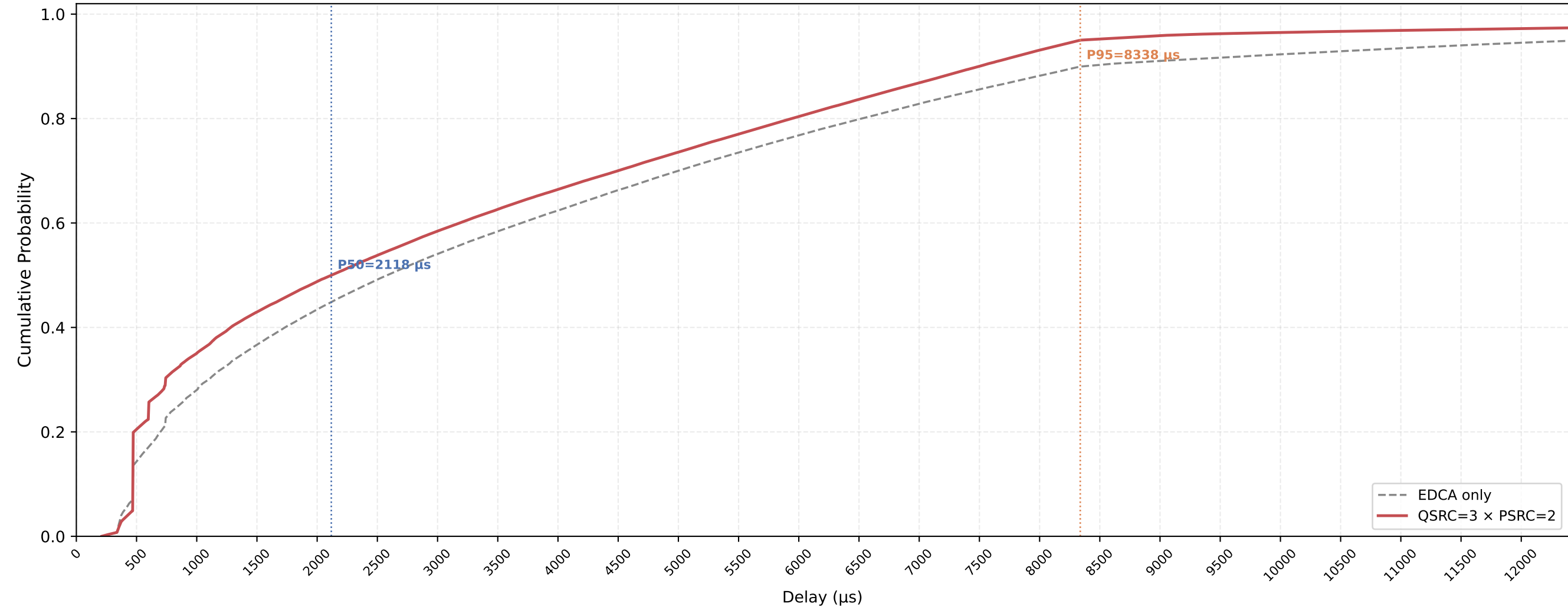
P-EDCA STA VO Delay CDF — QSRC=3 × PSRC=2 nSta=30, nPedca=30, 1Mbps, avg of 10 runs
