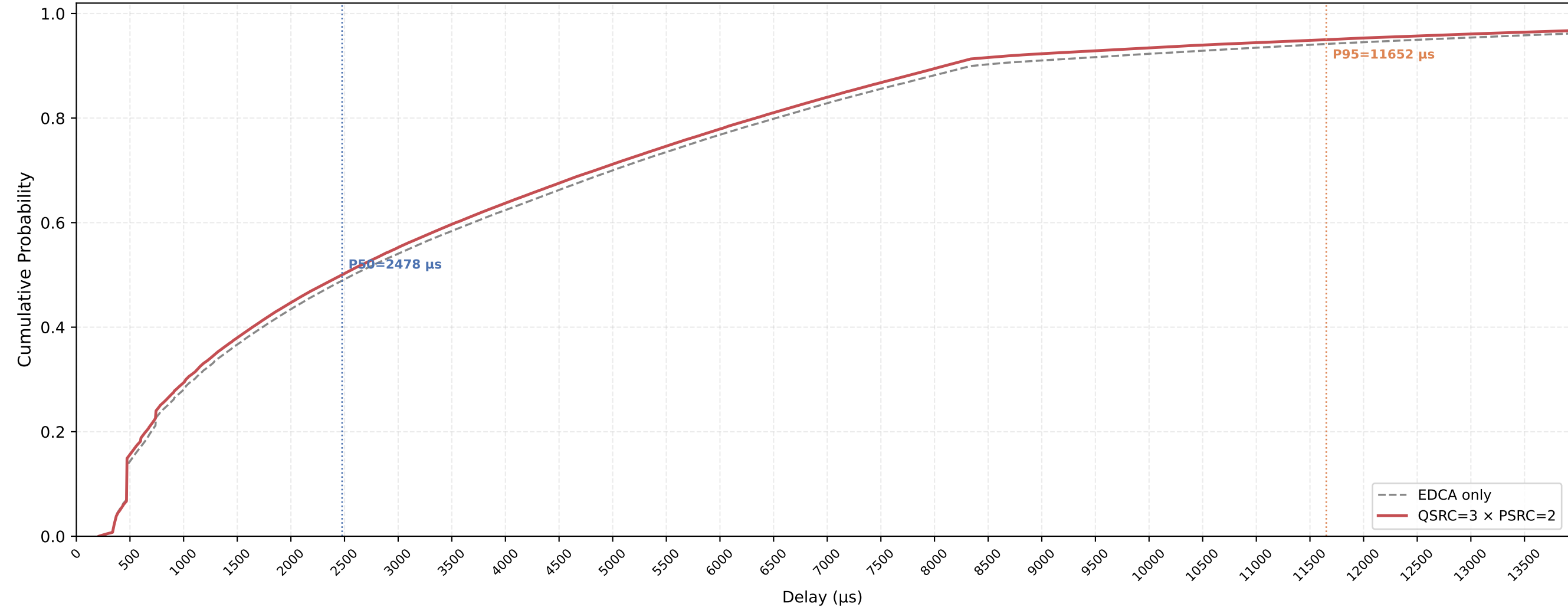
VO (all STAs) Delay CDF — QSRC=3 × PSRC=2 nSta=30, nPedca=5, 1Mbps, avg of 10 runs
