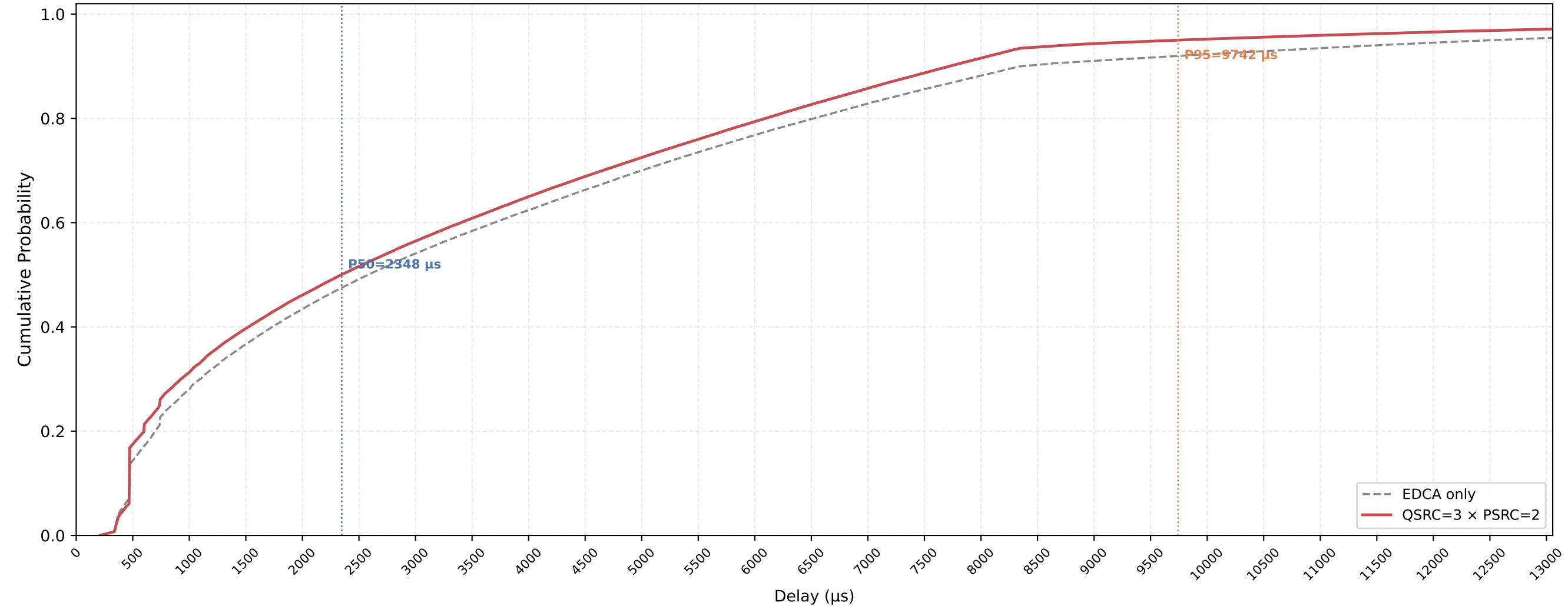
VO (all STAs) Delay CDF — QSRC=3 × PSRC=2 nSta=30, nPedca=15, 1Mbps, avg of 10 runs
