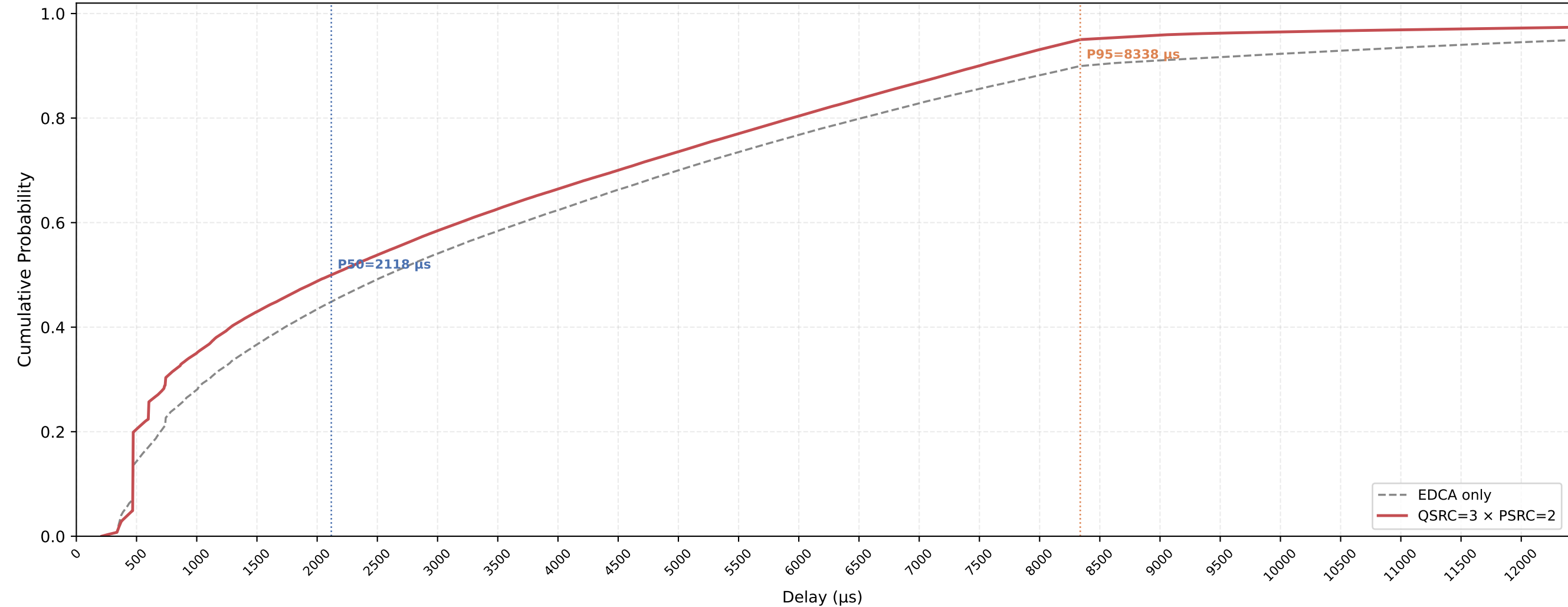
VO (all STAs) Delay CDF — QSRC=3 × PSRC=2 nSta=30, nPedca=30, 1Mbps, avg of 10 runs
