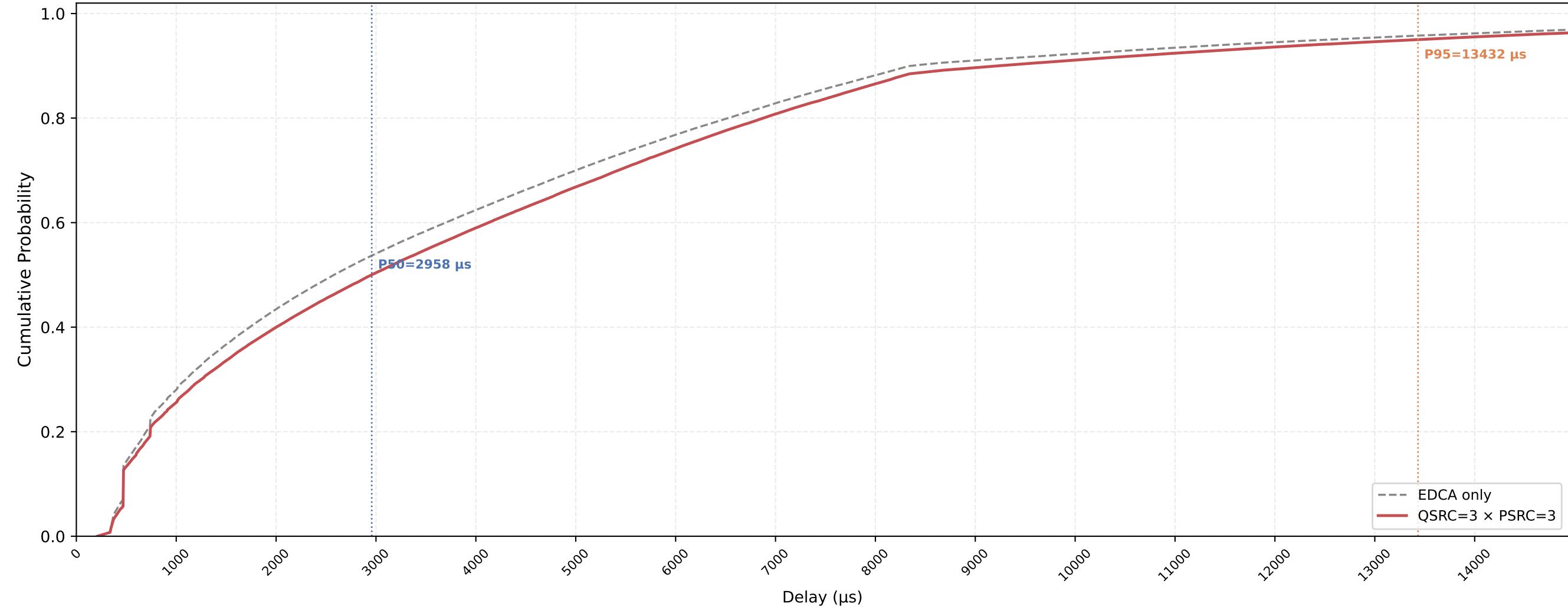
Legacy STA VO Delay CDF — QSRC=3 × PSRC=3 nSta=30, nPedca=15, 1Mbps, avg of 10 runs
