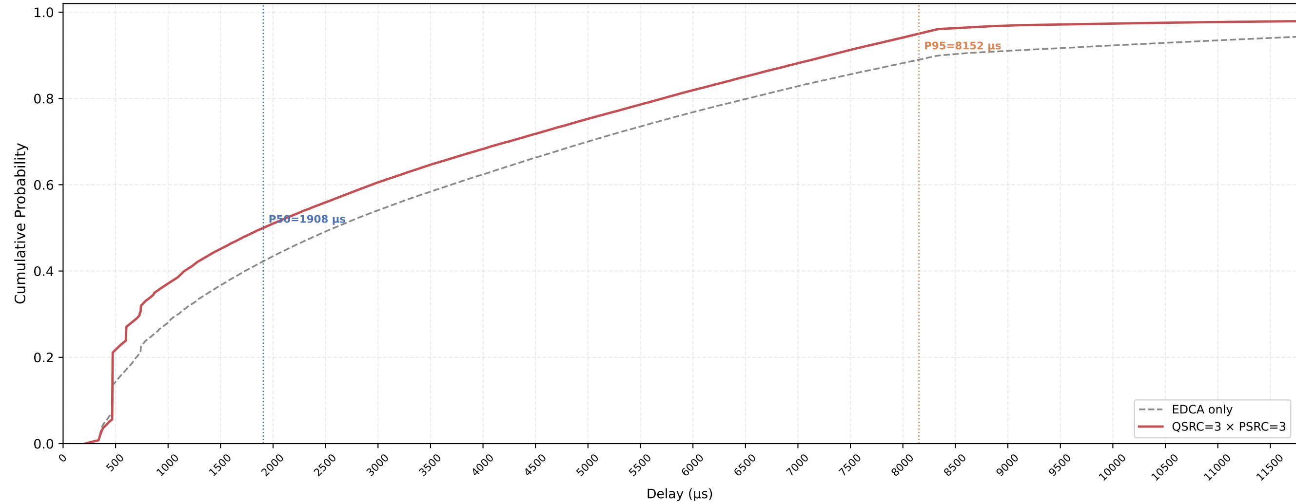
P-EDCA STA VO Delay CDF — QSRC=3 × PSRC=3 nSta=30, nPedca=15, 1Mbps, avg of 10 runs
